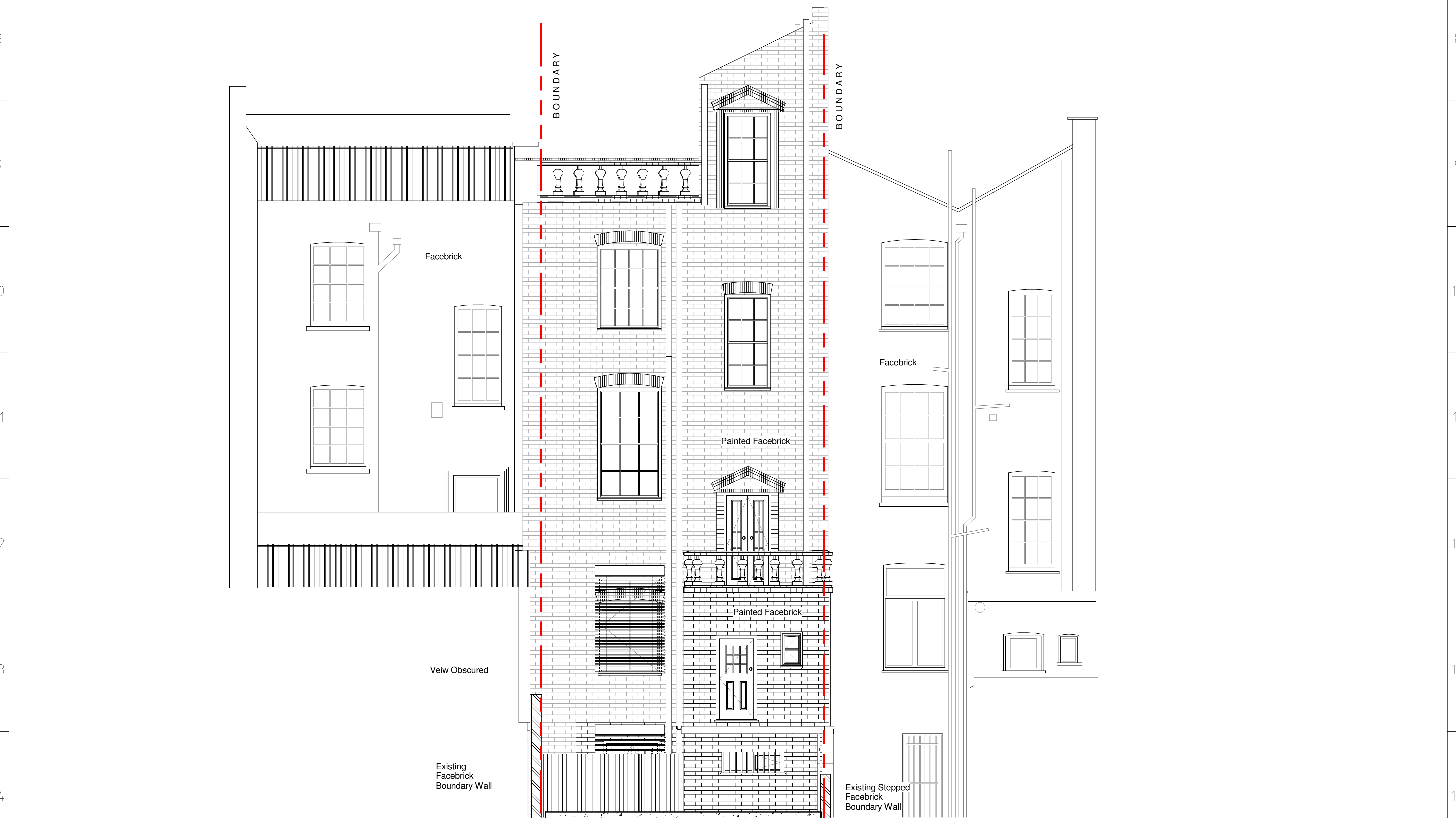
2 Existing Rear Elevation 1 : 50
