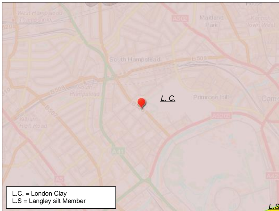
Figure 2. Superficial and Bedrock geology of the Site (Ref. BGS Geindex)
