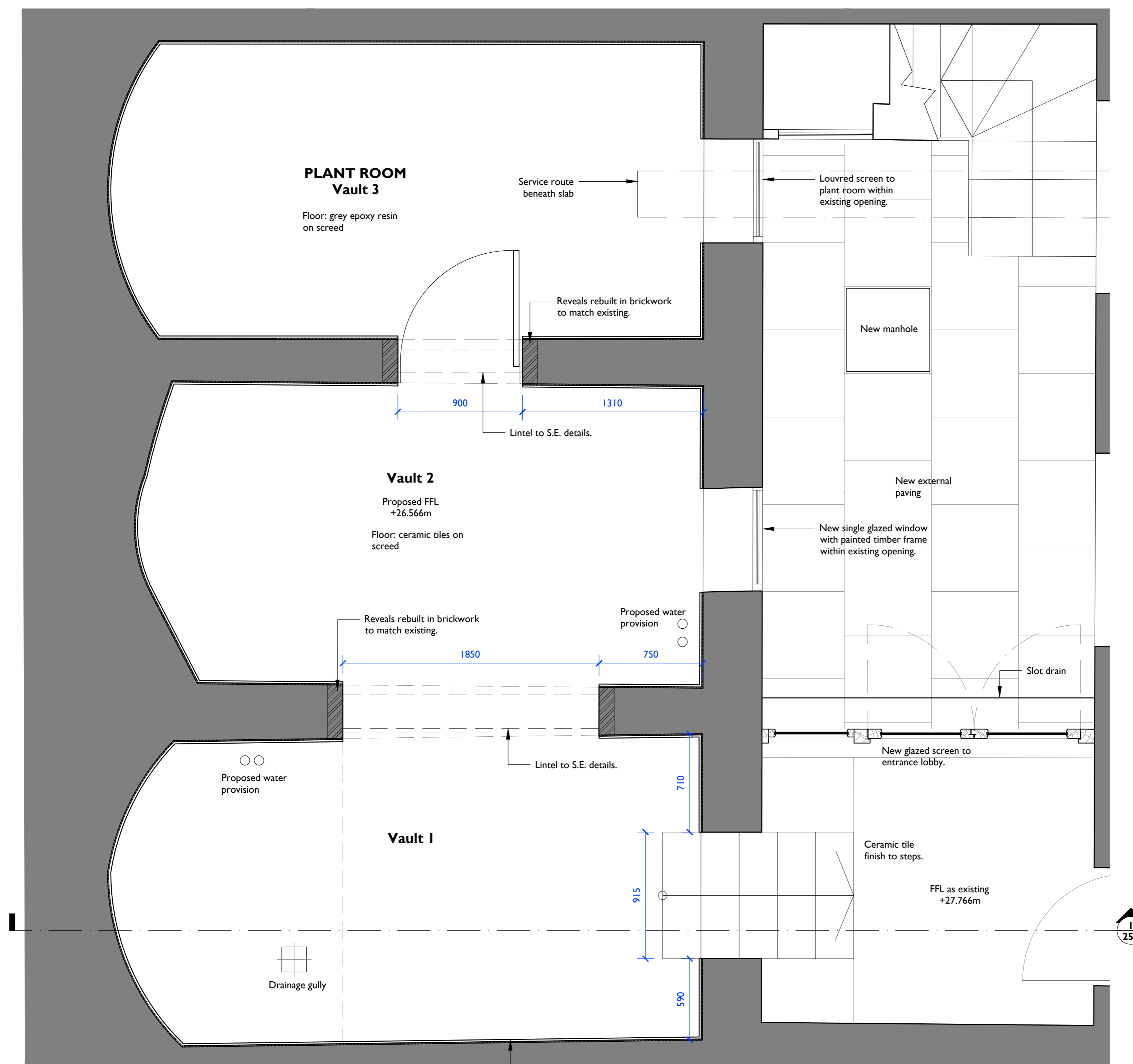
2 PROPOSED VAULT PLAN 250 1:20 at A1
