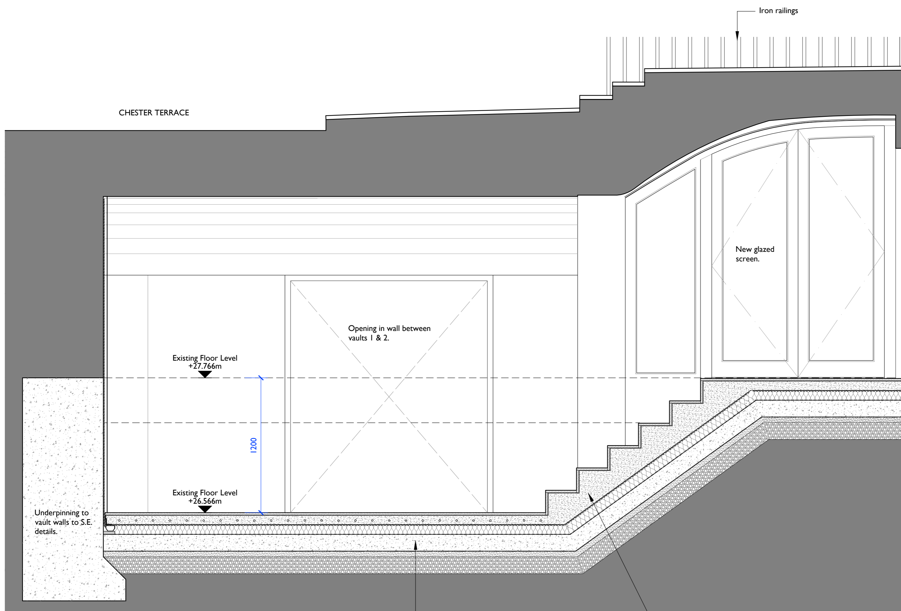
1 SECTION AA 250 1:20 at A1
