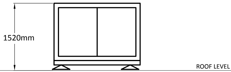
BOOSTER SET GRP HOUSING ELEVATION (1:50@ A1)
