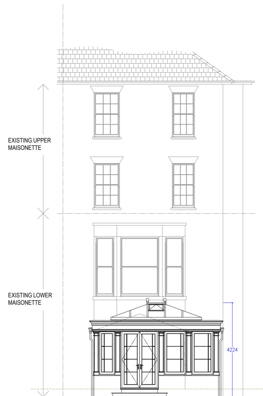
PROPOSED REAR ELEVATION Scale 1:100
