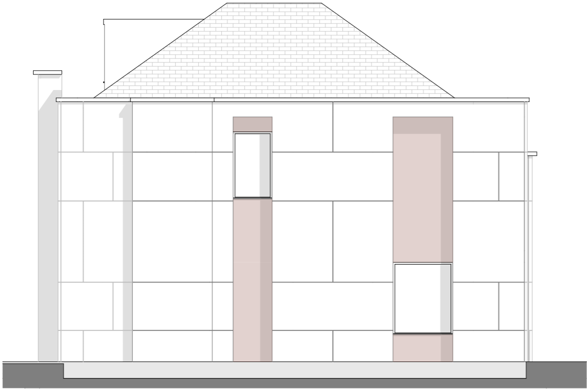
E-03 Side Elevation 01 (East) 1:100
