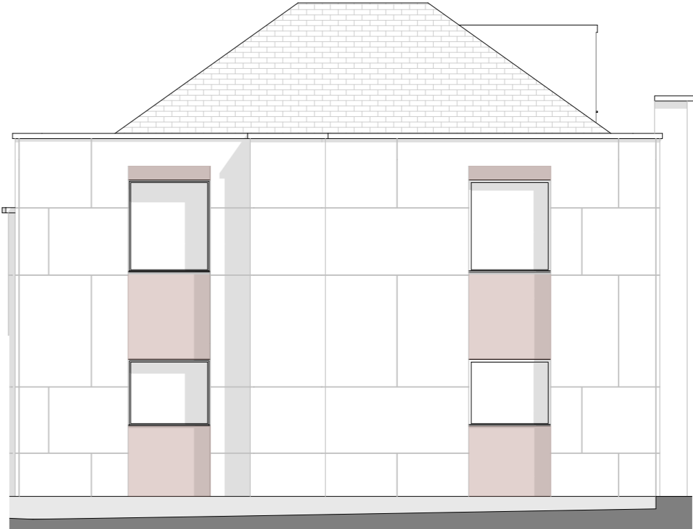
E-04 Side Elevation 02 (West) 1:100
