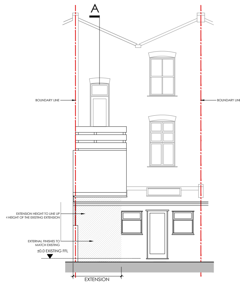
3 ELEVATION-REAR - PROPOSED 1:100
