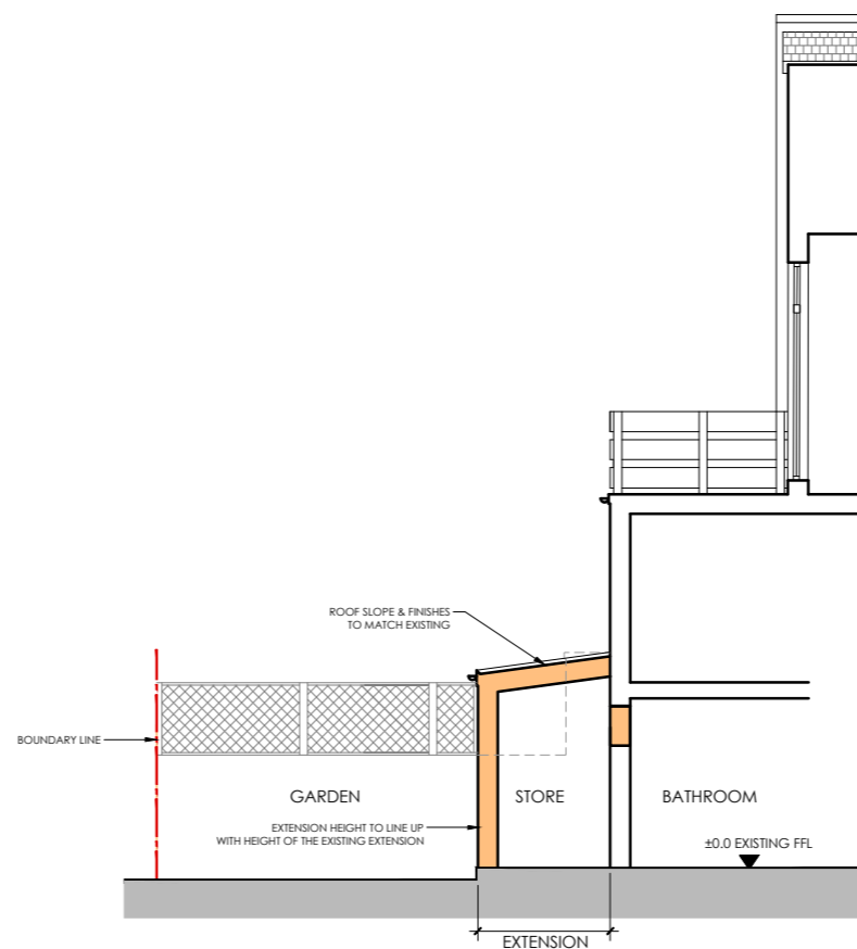
4 SECTION - A - PROPOSED 1:100
