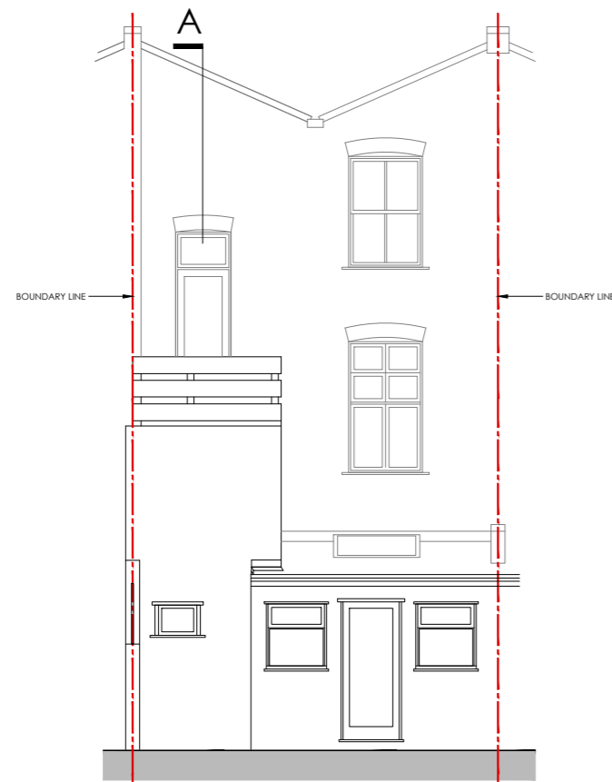
1 ELEVATION-REAR - EXISTING 1:100
