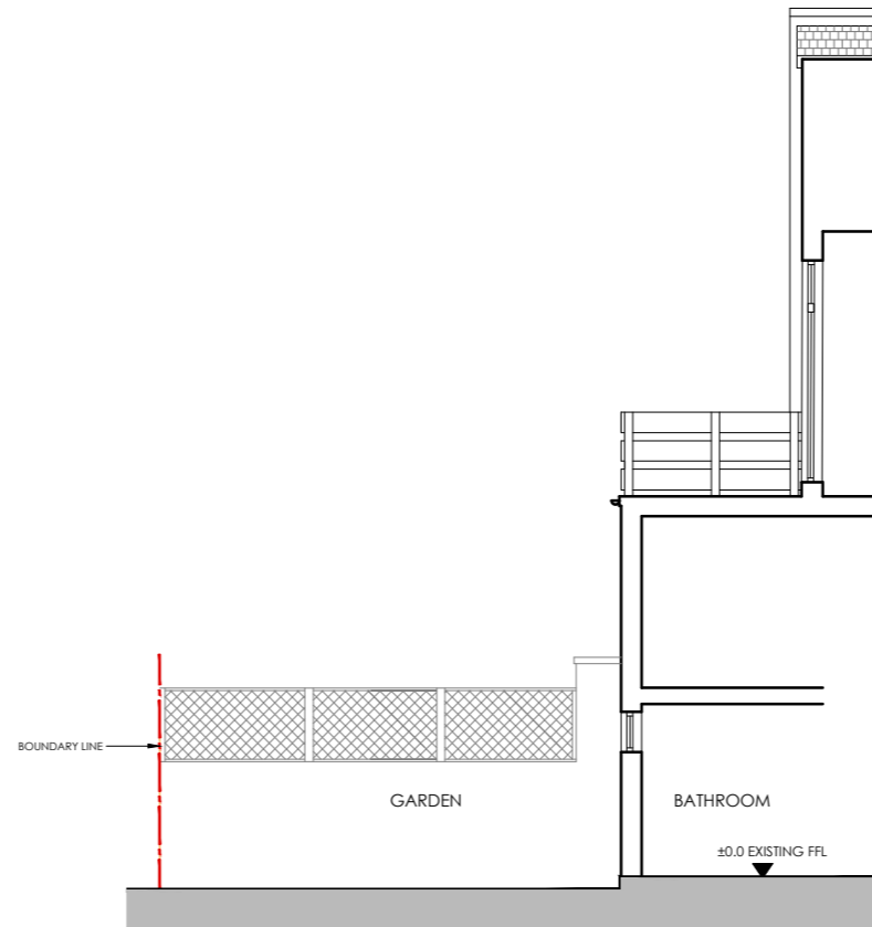
2 SECTION - A - EXISTING 1:100
