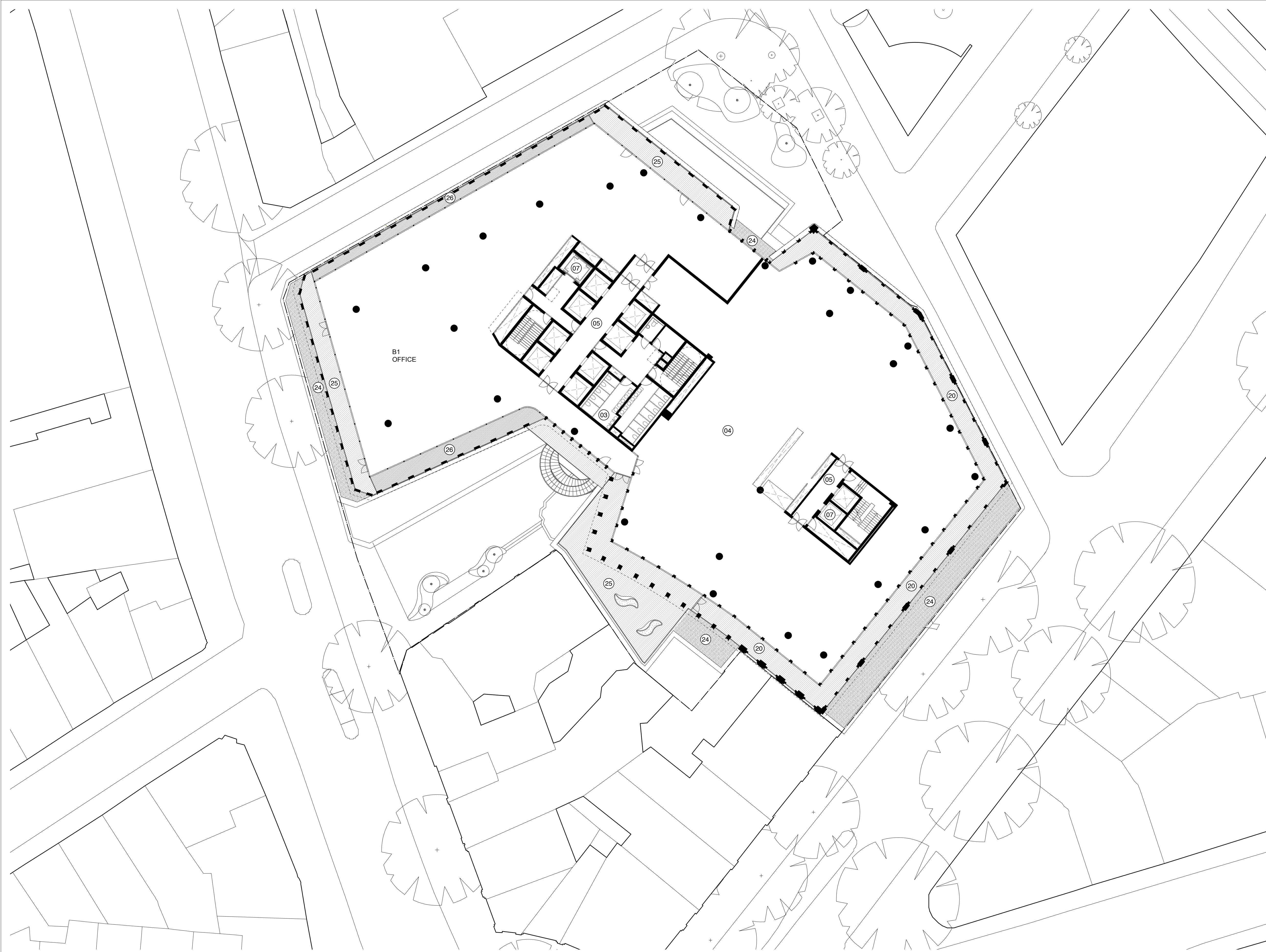
1 Proposed Seventh Floor Plan 1:200 @ A1
