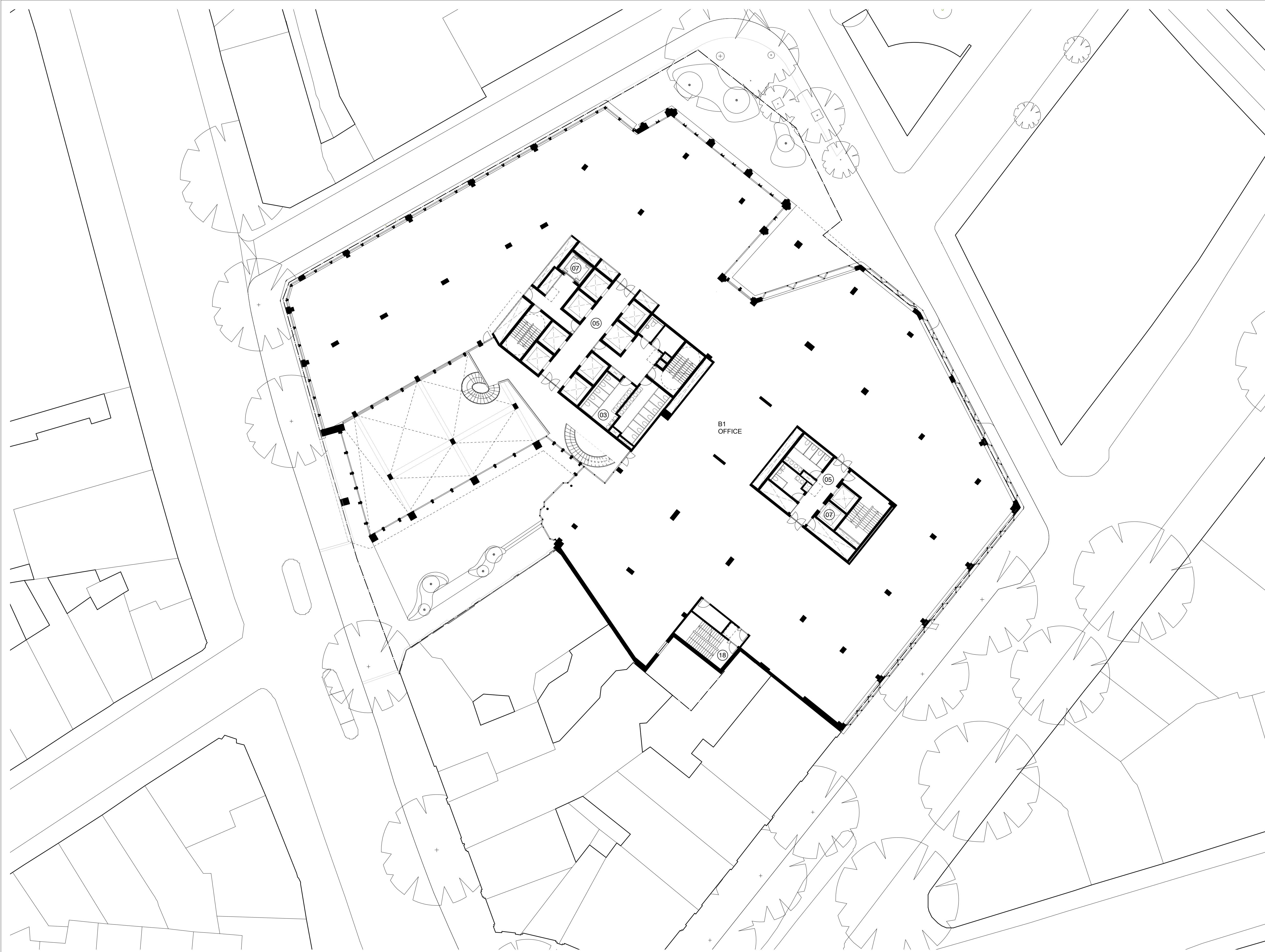
1 Proposed First Floor Plan 1:200 @ A1
