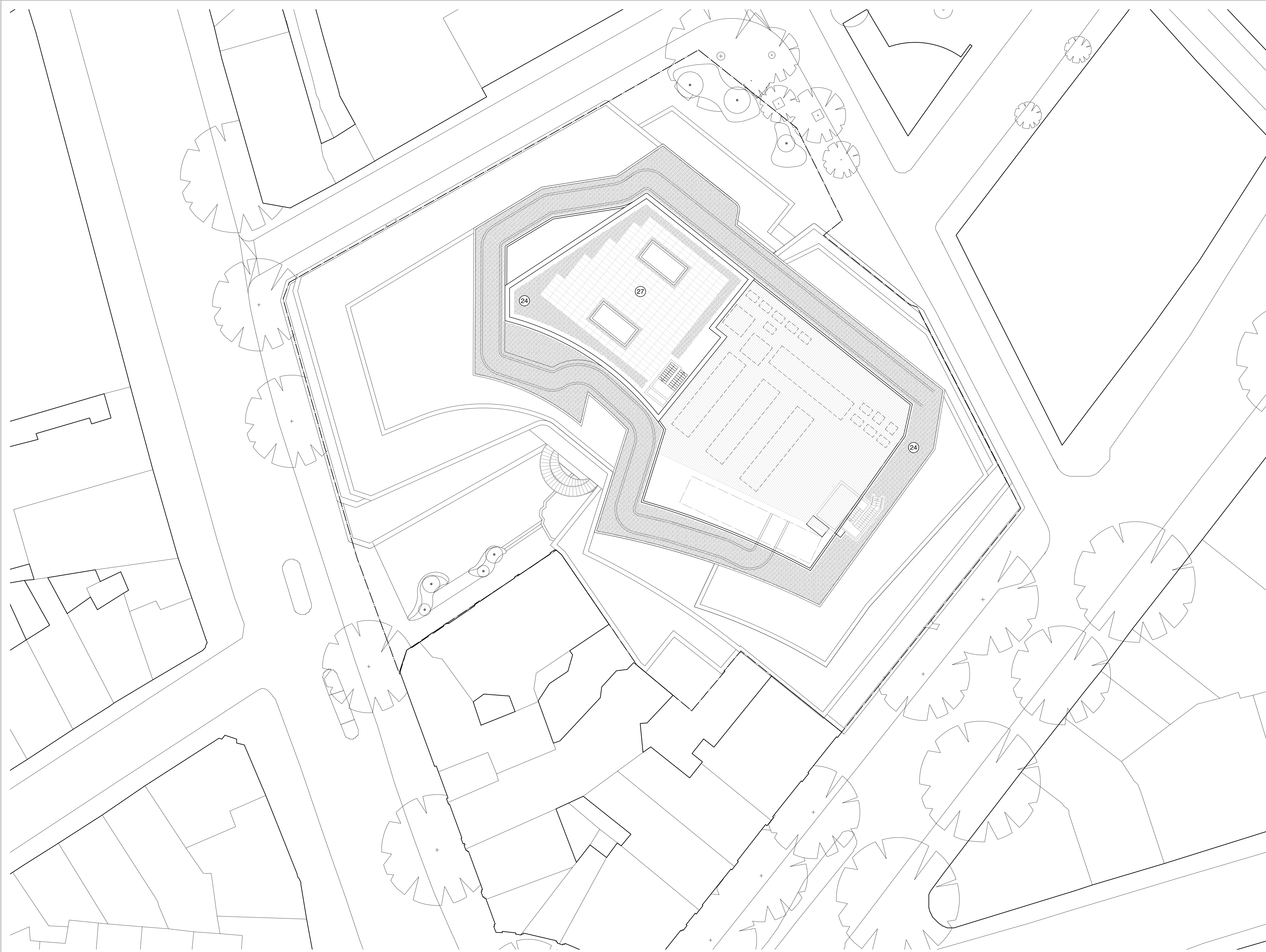
1 Proposed Roof Plan 1:200 @ A1
