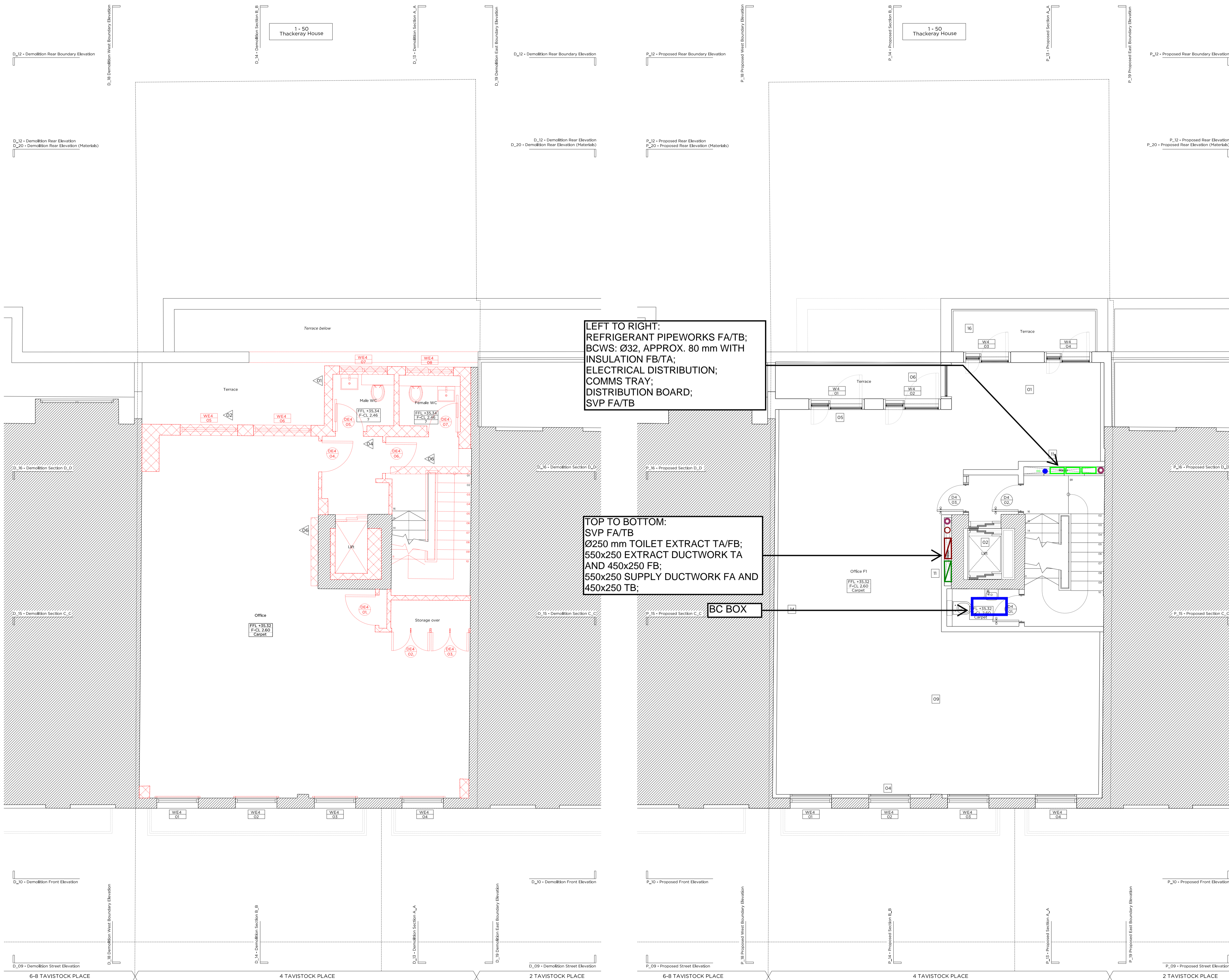
Demolition Fourth Floor Plan
