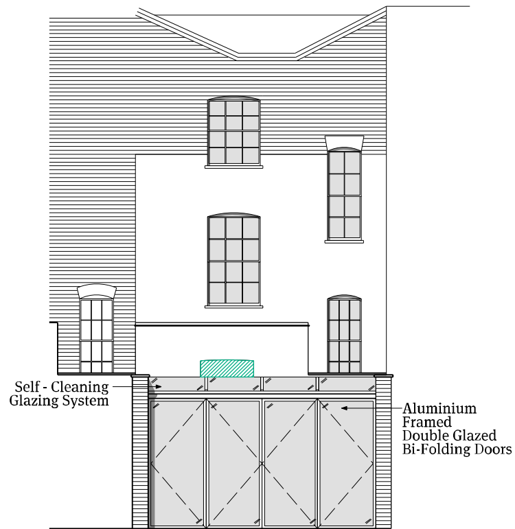
03 Proposed Rear Elevation 1:100@A3
