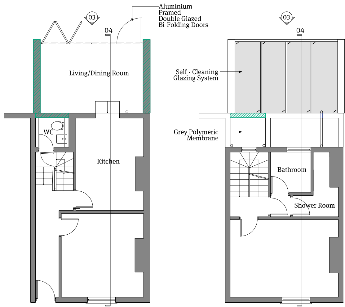
01 Proposed Ground Floor 1:100@A3
