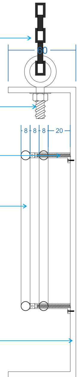
Sign Section Scale 1:2
