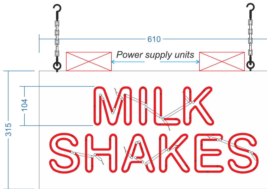
Internal Neon Milkshake Sign Scale 1:5
