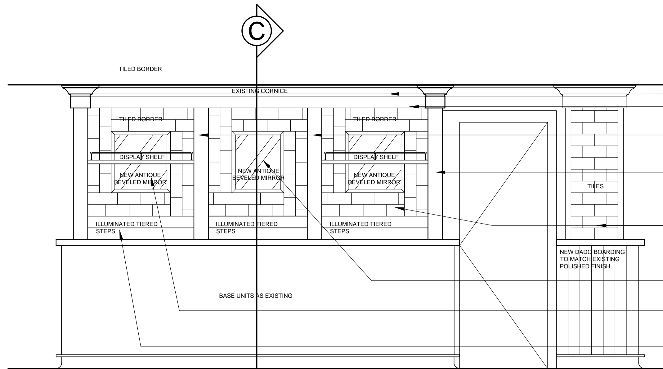
ELEVATION A SCALE 1:20
