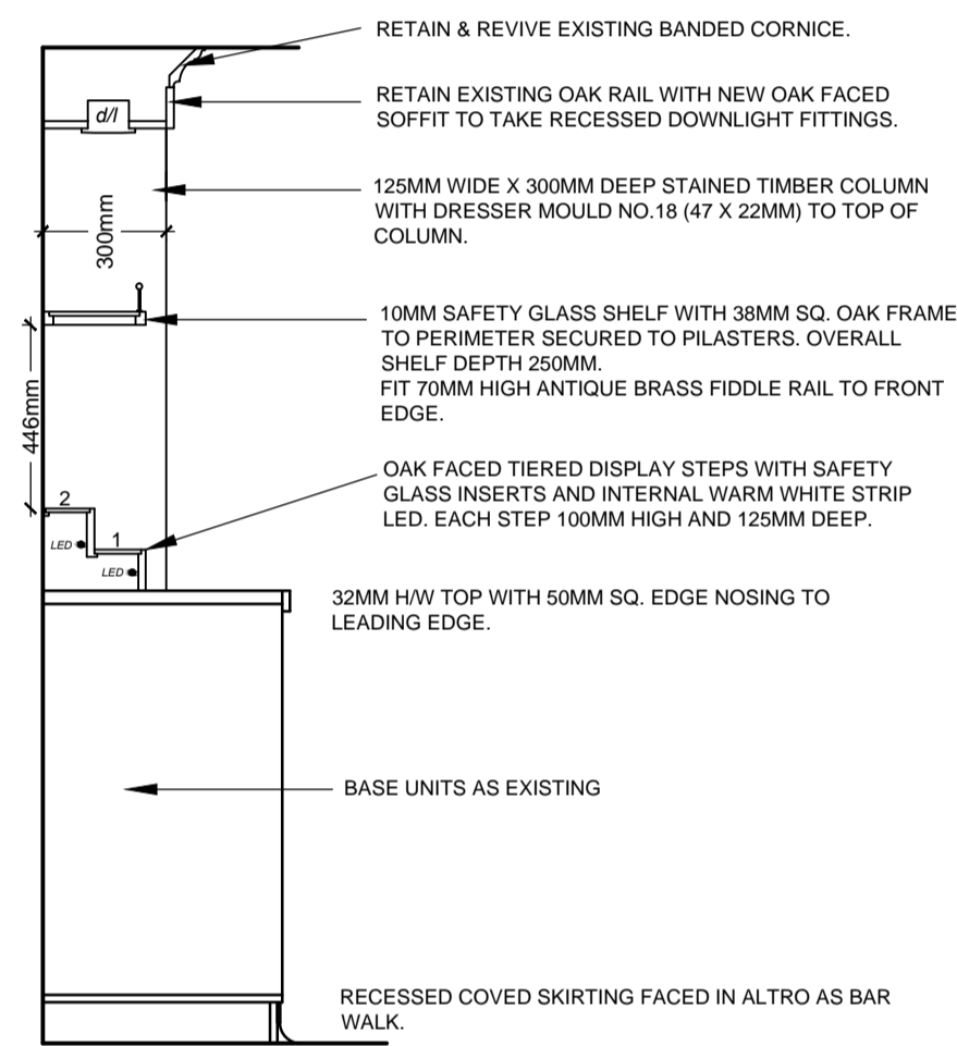
SECTION CC SCALE 1:20
