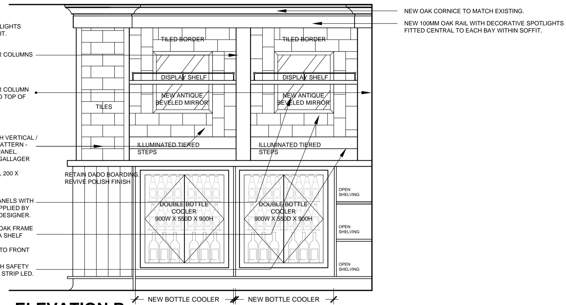
ELEVATION B SCALE 1:20
