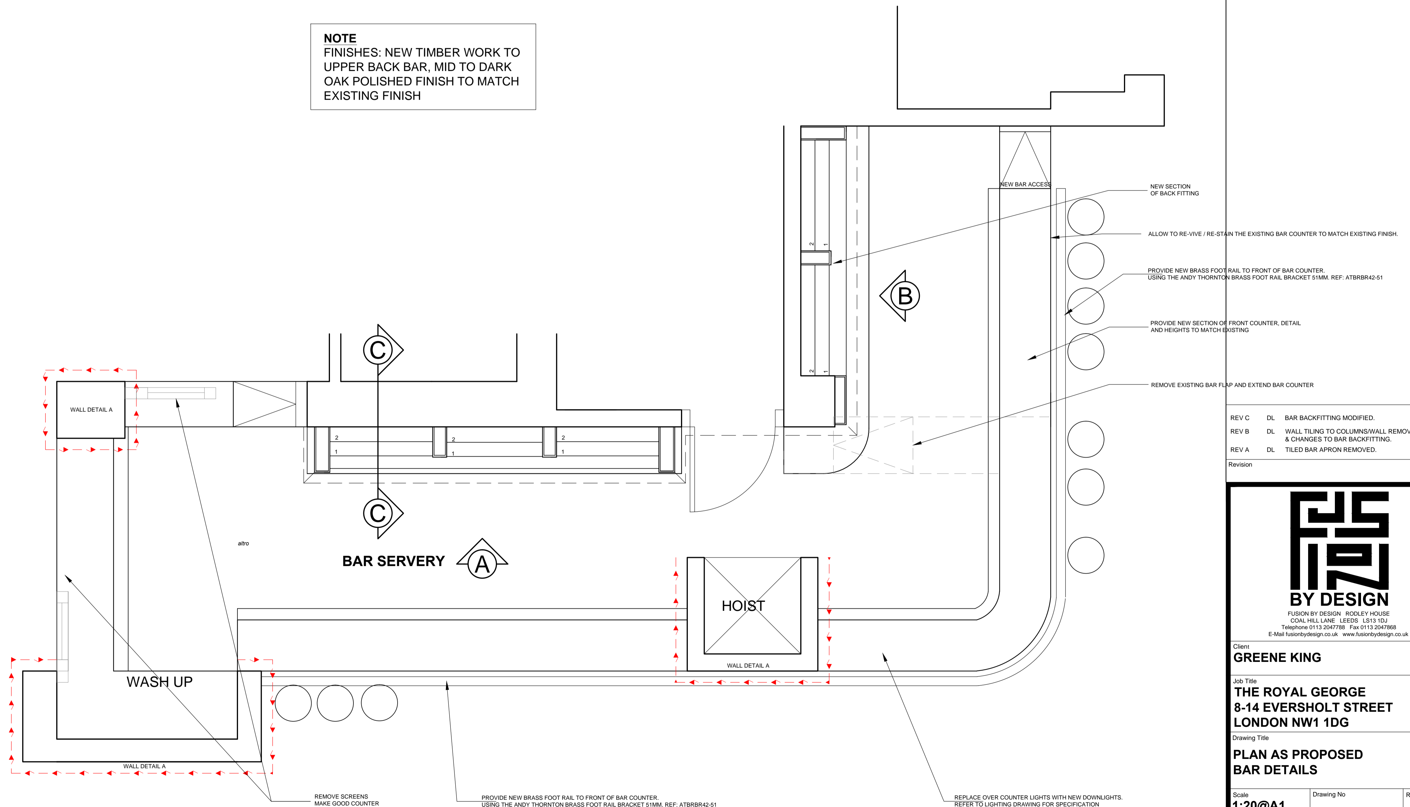
BAR COUNTER PLAN SCALE 1:20
