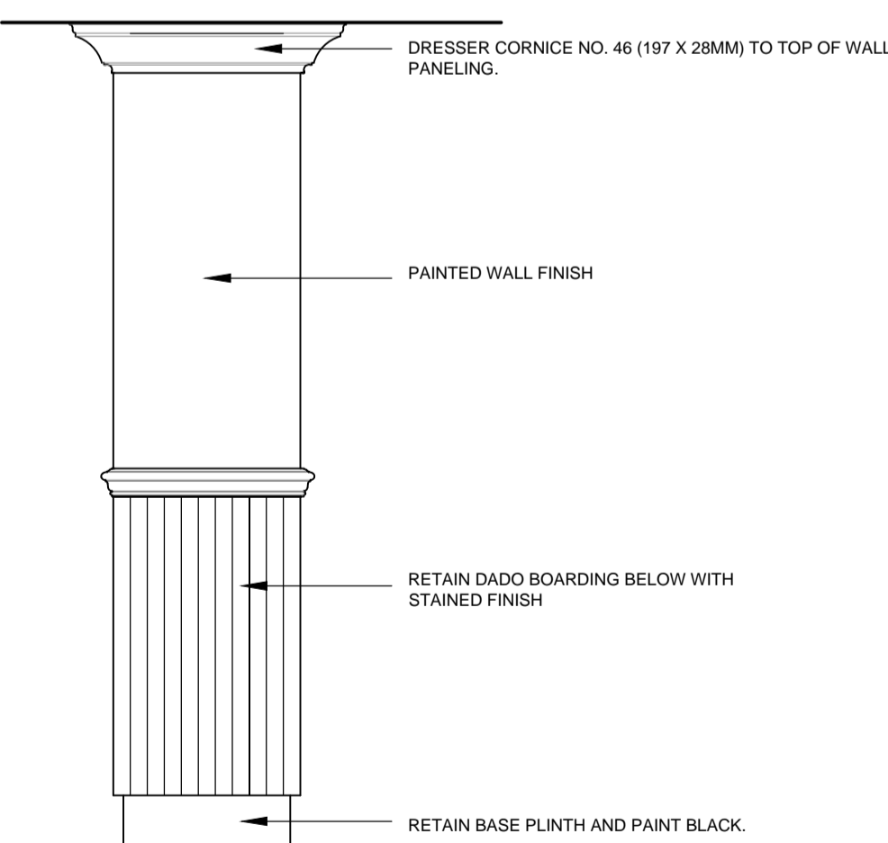
WALL DETAIL A SCALE 1:20
