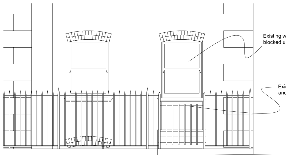
Elevation of Blocked up Door Opening As Existing 1:25
