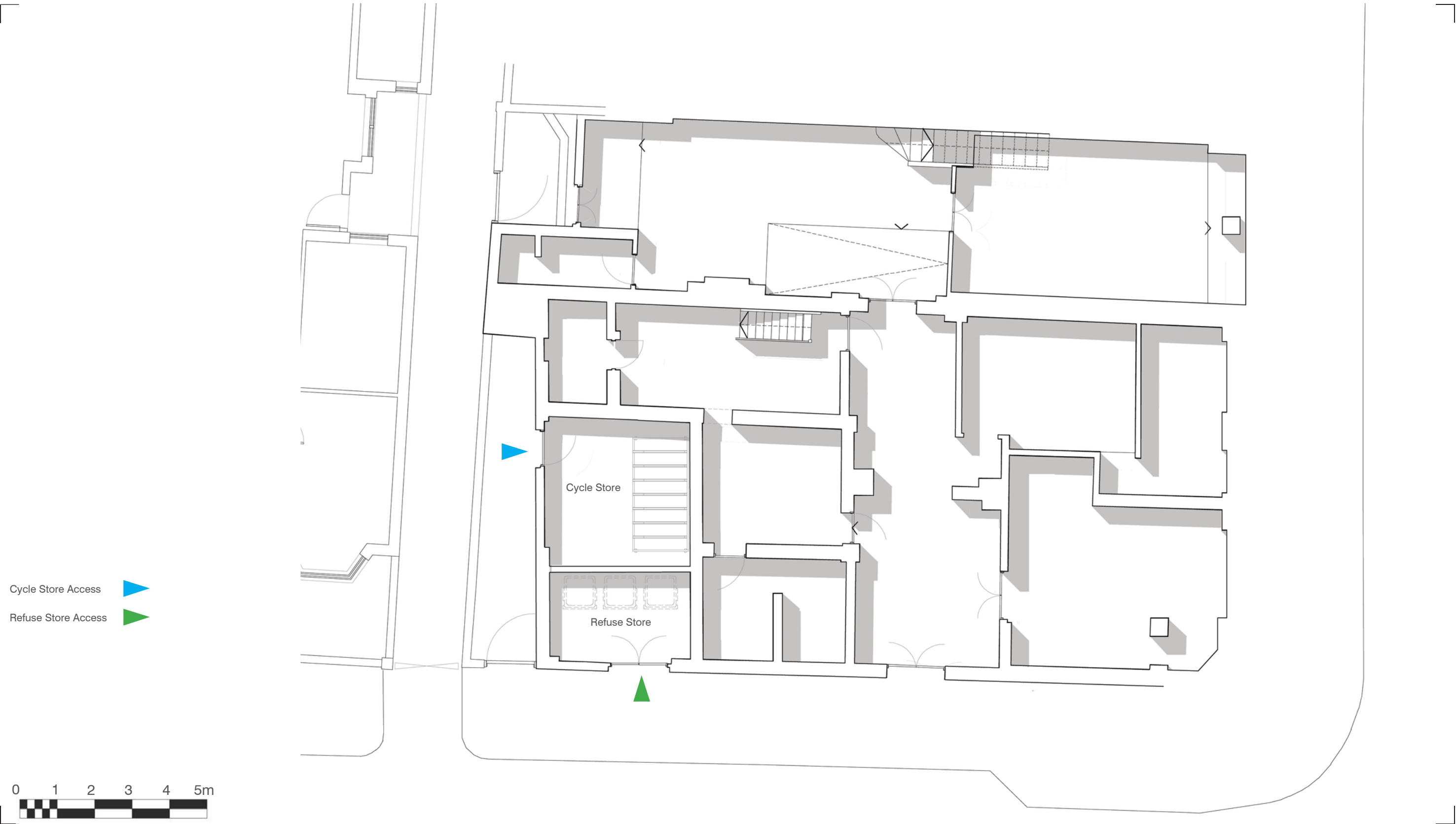
LOWER GROUND FLOOR PLAN. DRAWING no. 2000B. 1:100@A3
