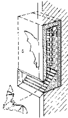
[Pic. 8]: 1FE with the optional Back Plate with integrated wooden panel for bats to cling on. Example for installation in wall
