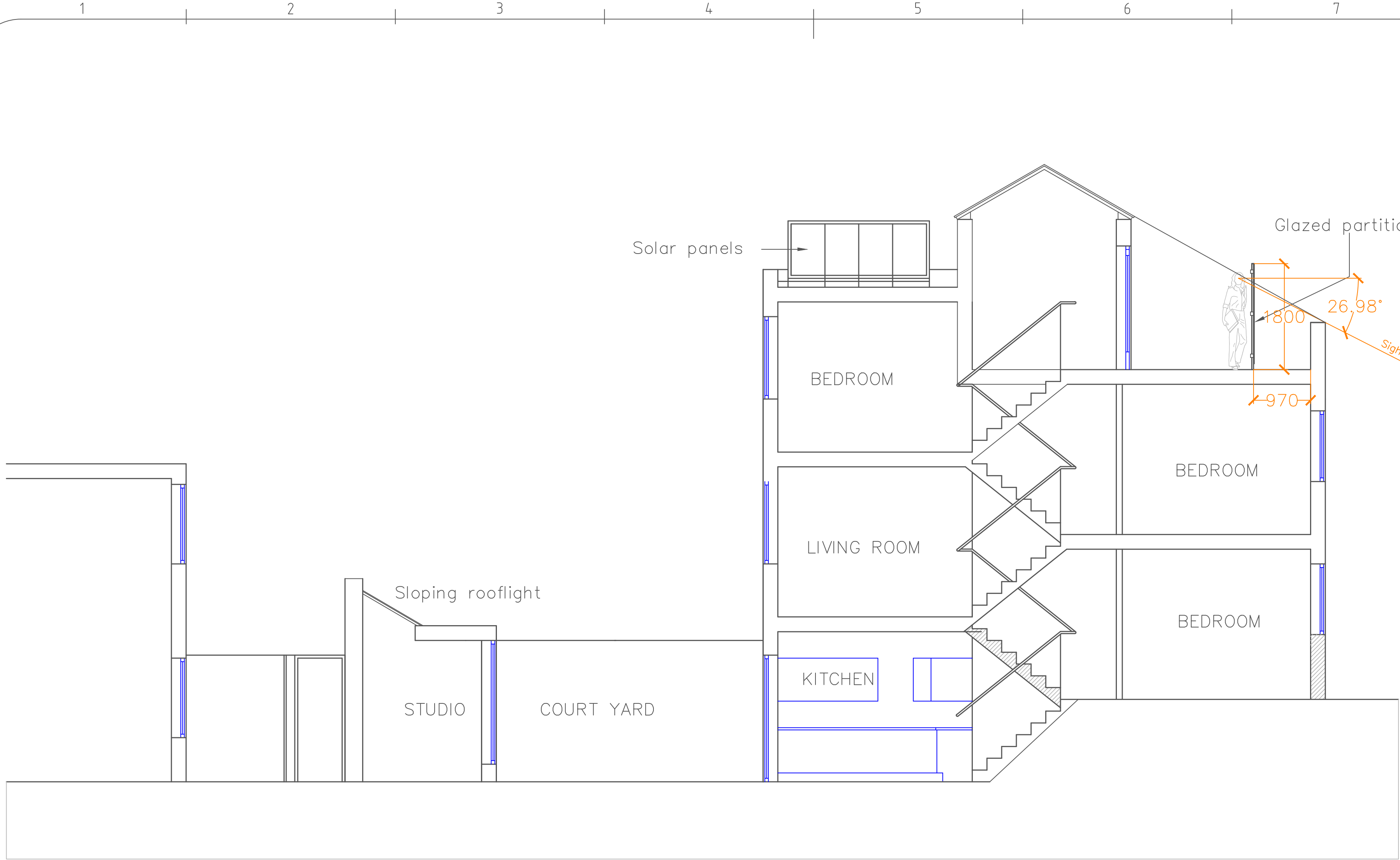
LONG SECTION
