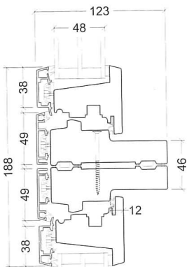
Transom, opening sashes
