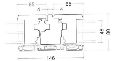
Mullion with French casement
