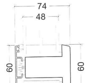
60mm glazing bar
