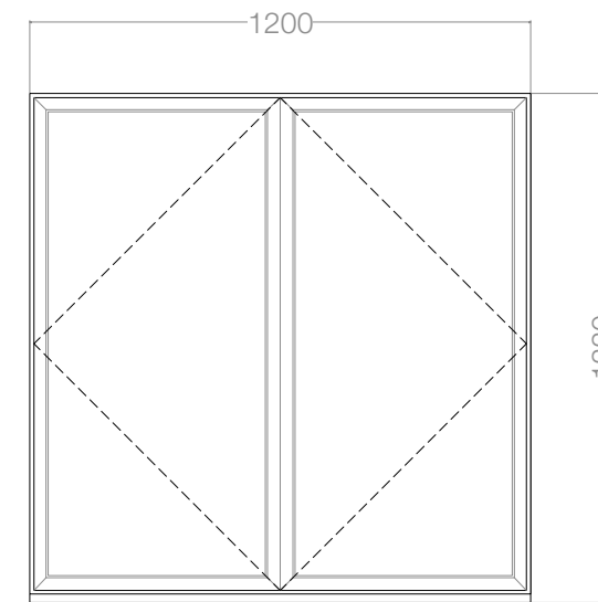
EW16 1:20 @ A1
