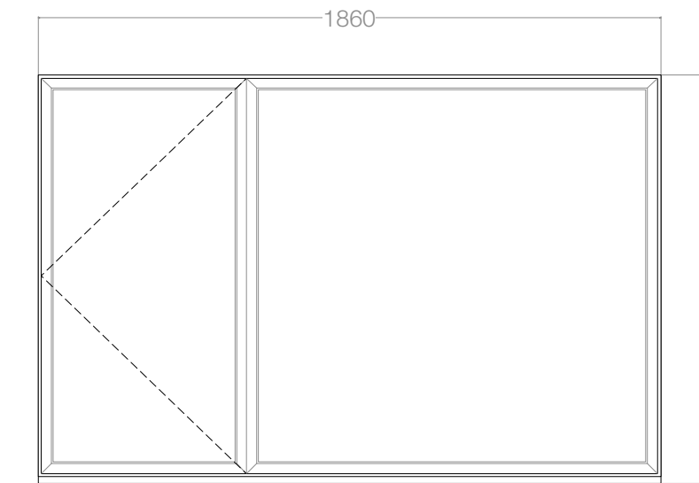
EW17 1:20 @ A1
