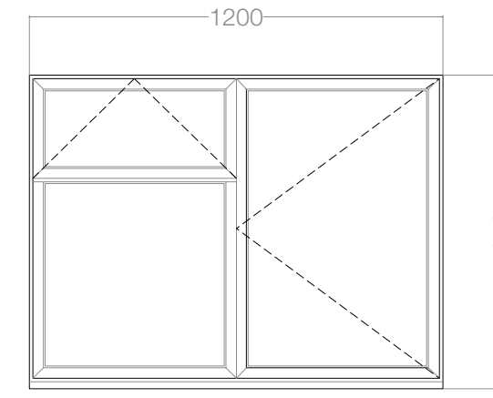
EW3 1:20 @ A1
