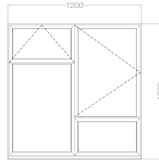
EW4 1:20 @ A1
