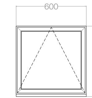
EW12 1:20 @ A1
