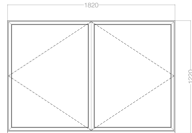
EW14 1:20 @ A1
