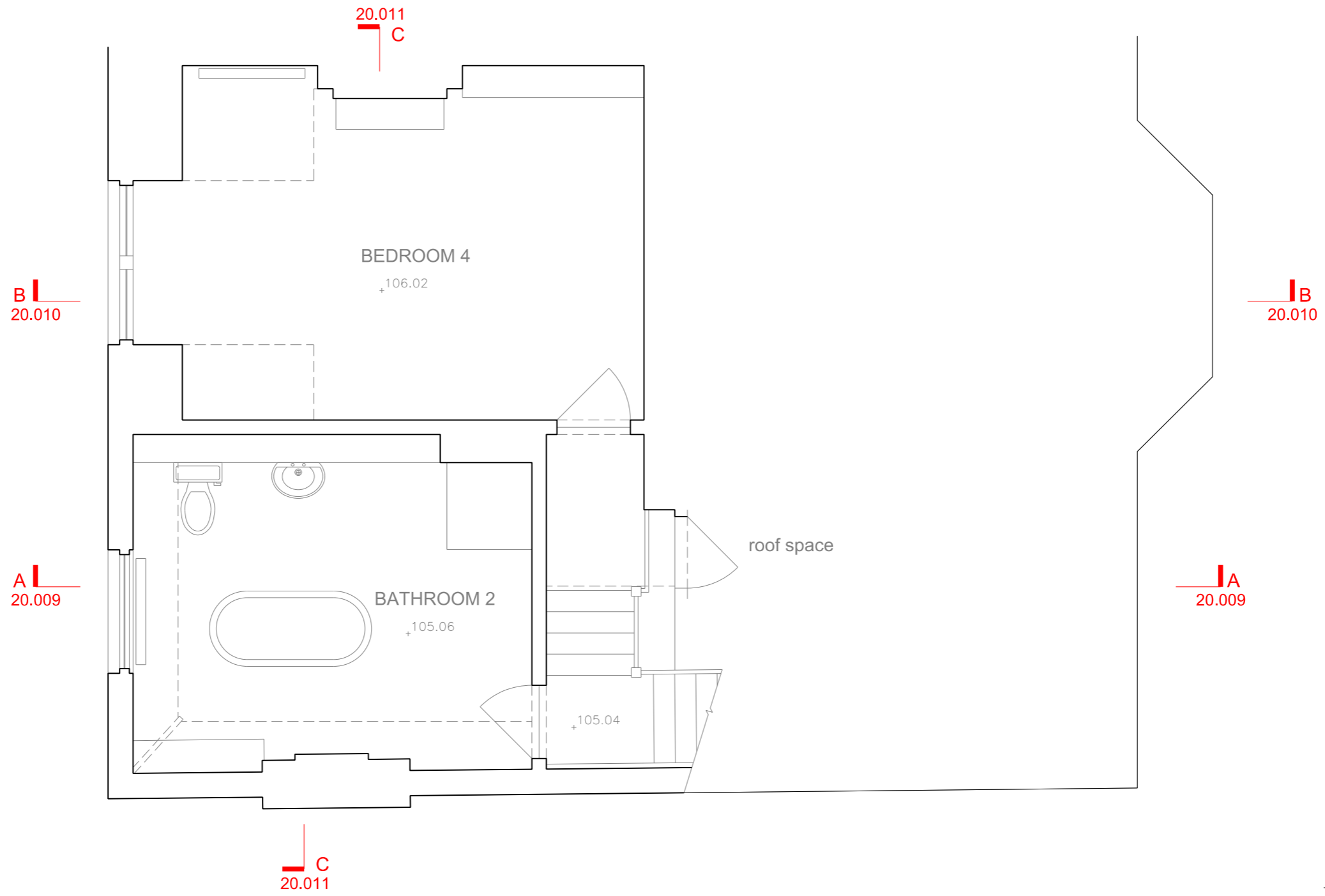
1 EXISTING SECOND FLOOR PLAN
