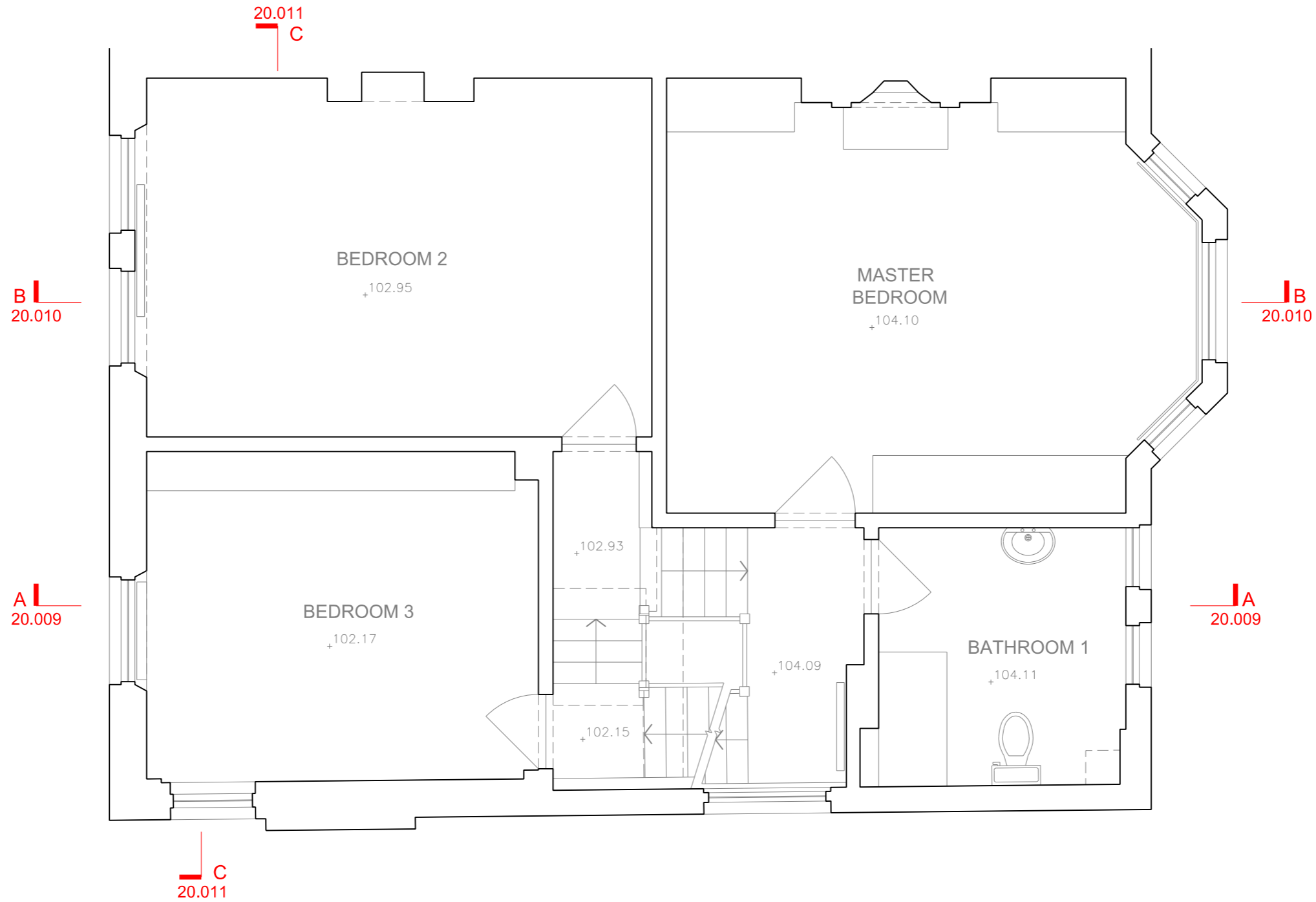
1 EXISTING FIRST FLOOR PLAN
