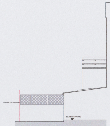
2 ELEVATION-SIDE (SOUTH EAST) - EXISTING 1:100
