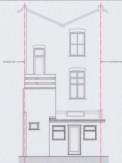
1 ELEVATION-REAR - EXISTING 1:100
