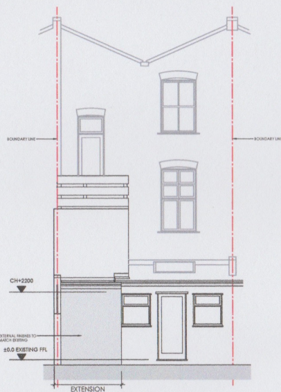
3 ELEVATION-REAR - PROPOSED 1:100
