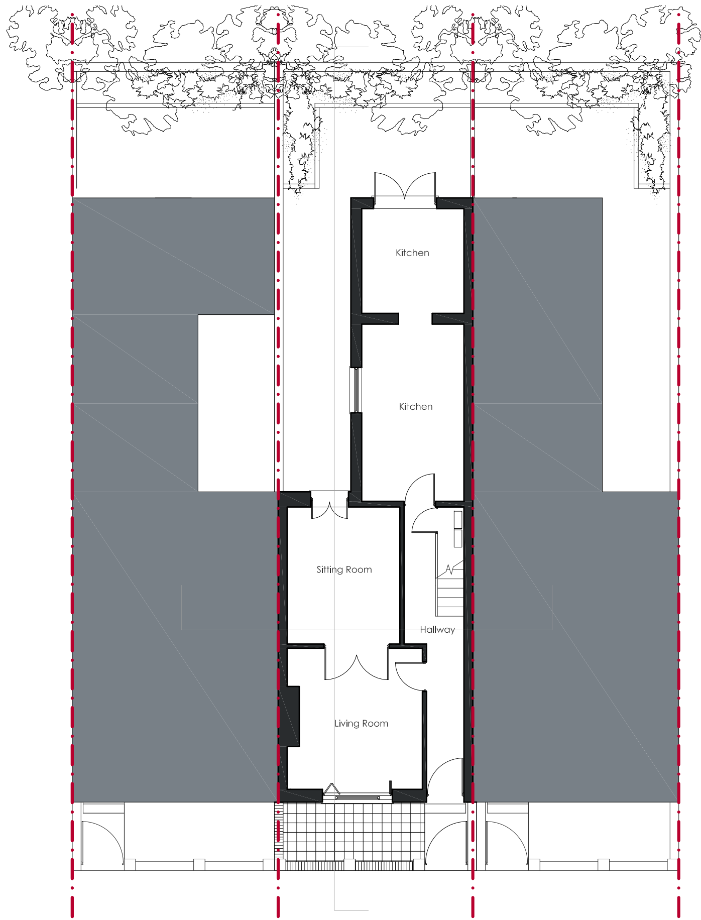
GROUND FLOOR
