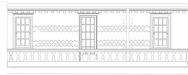
EXISTING TERRACE 1 BALUSTRADE ELEVATION SOUTH WEST WEST
