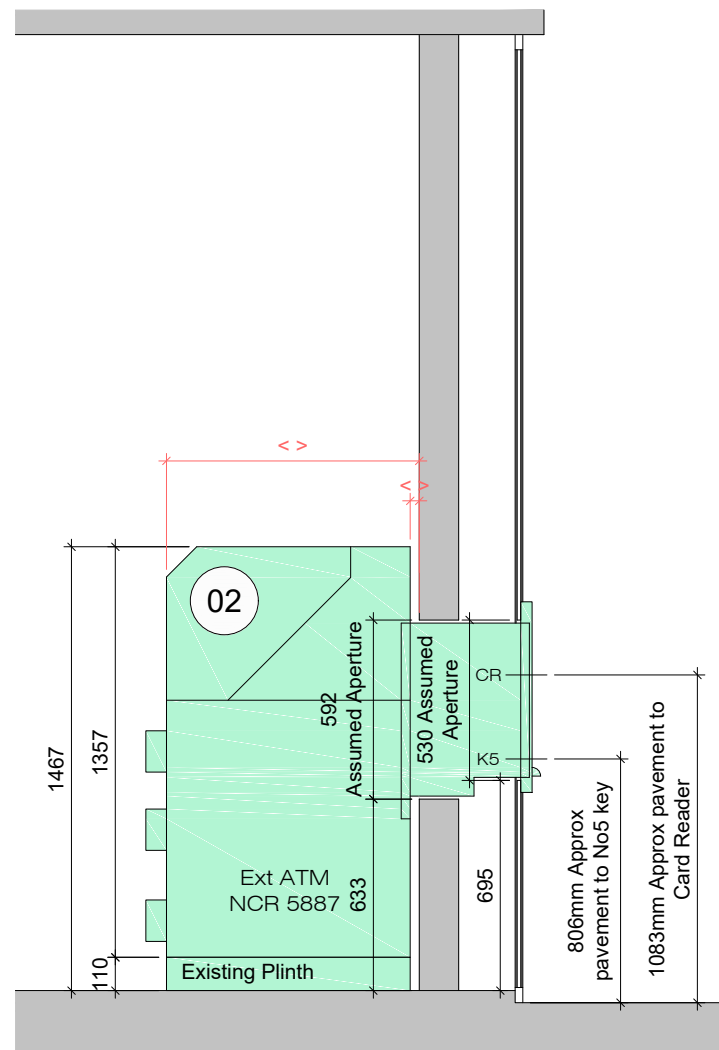
Existing Section - ATM2 (scale 1:25 @ A3)
