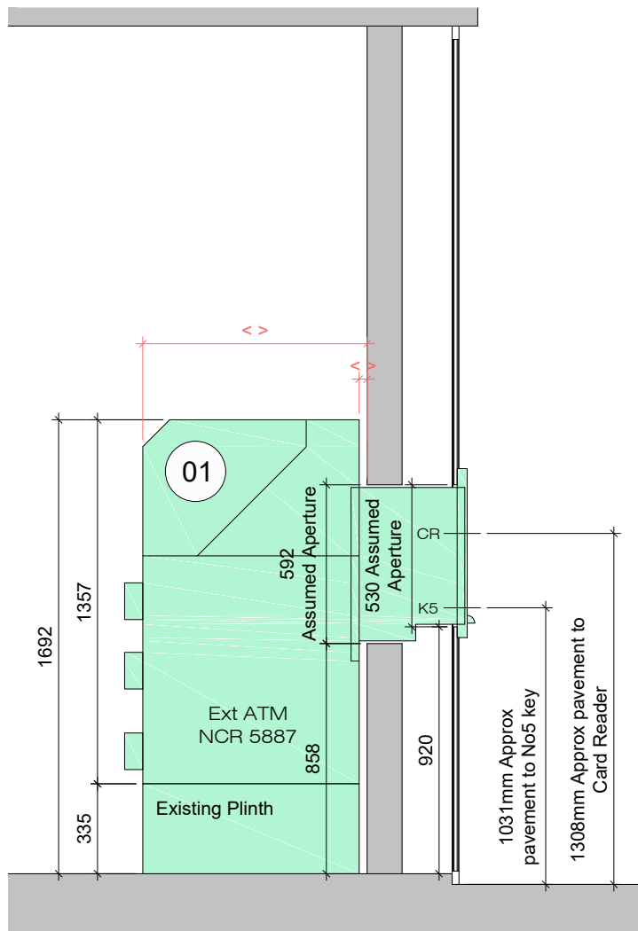
Existing Section - ATM1 (scale 1:25 @ A3)
