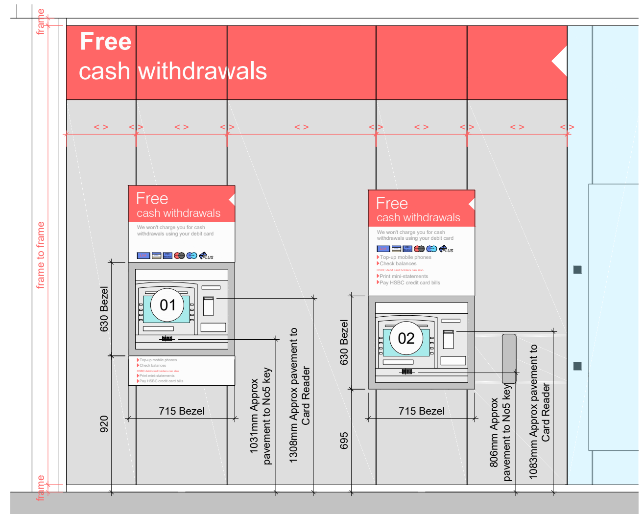
Existing Elevation (scale 1:25 @ A3)
