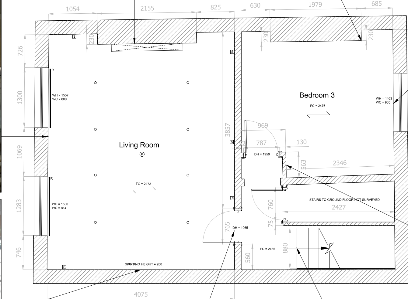
1 Existing First Floor Plan 1:50
