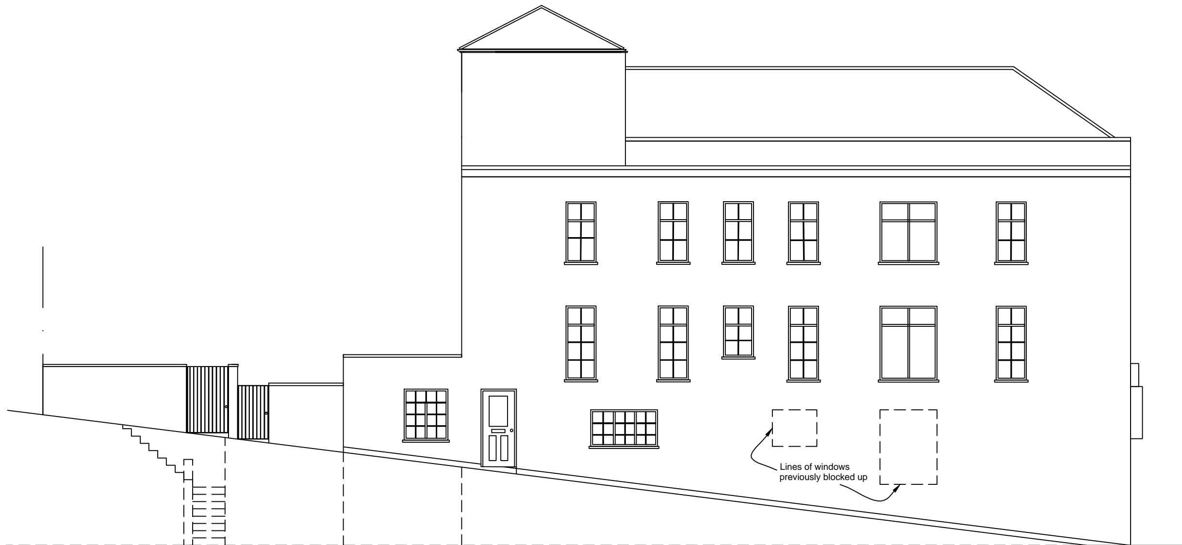
Proposed Side Elevation( Approved) 1:100
