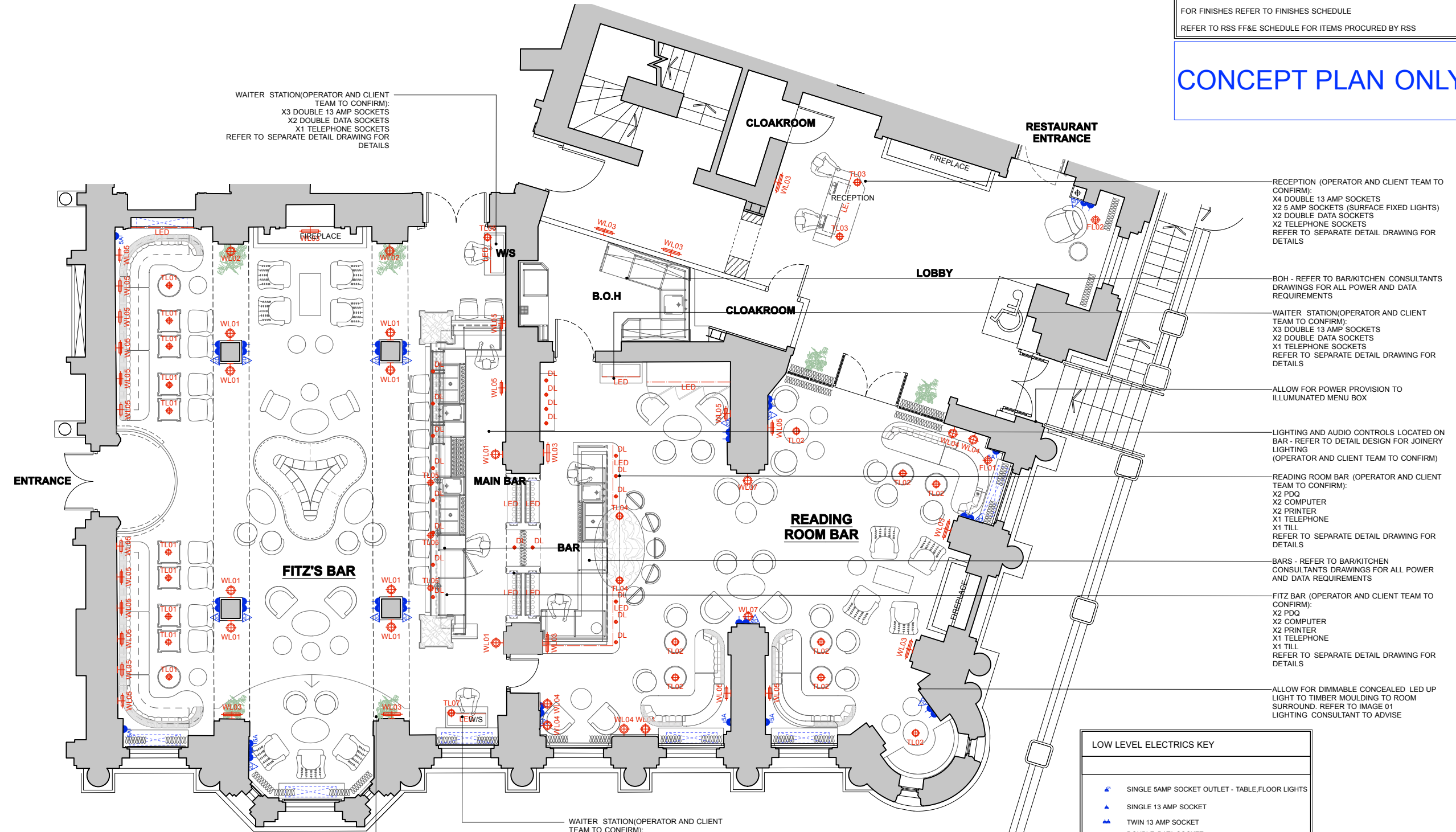
1 PL-03 GROUND FLOOR LOW LEVEL LIGHTING & ELECTRICS PLAN Scale: 1:50
