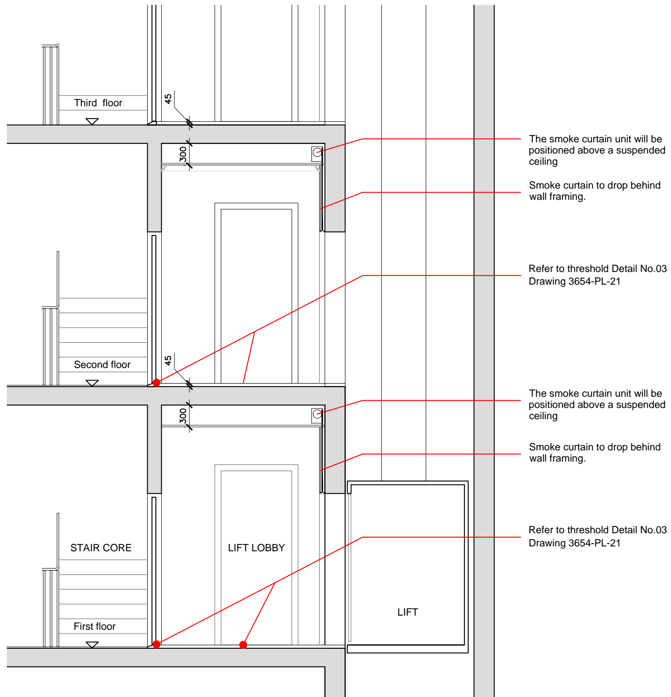
DETAIL 1 - SECTION THROUGH LIFT SHAFT/ LIFT LOBBY 1:50
