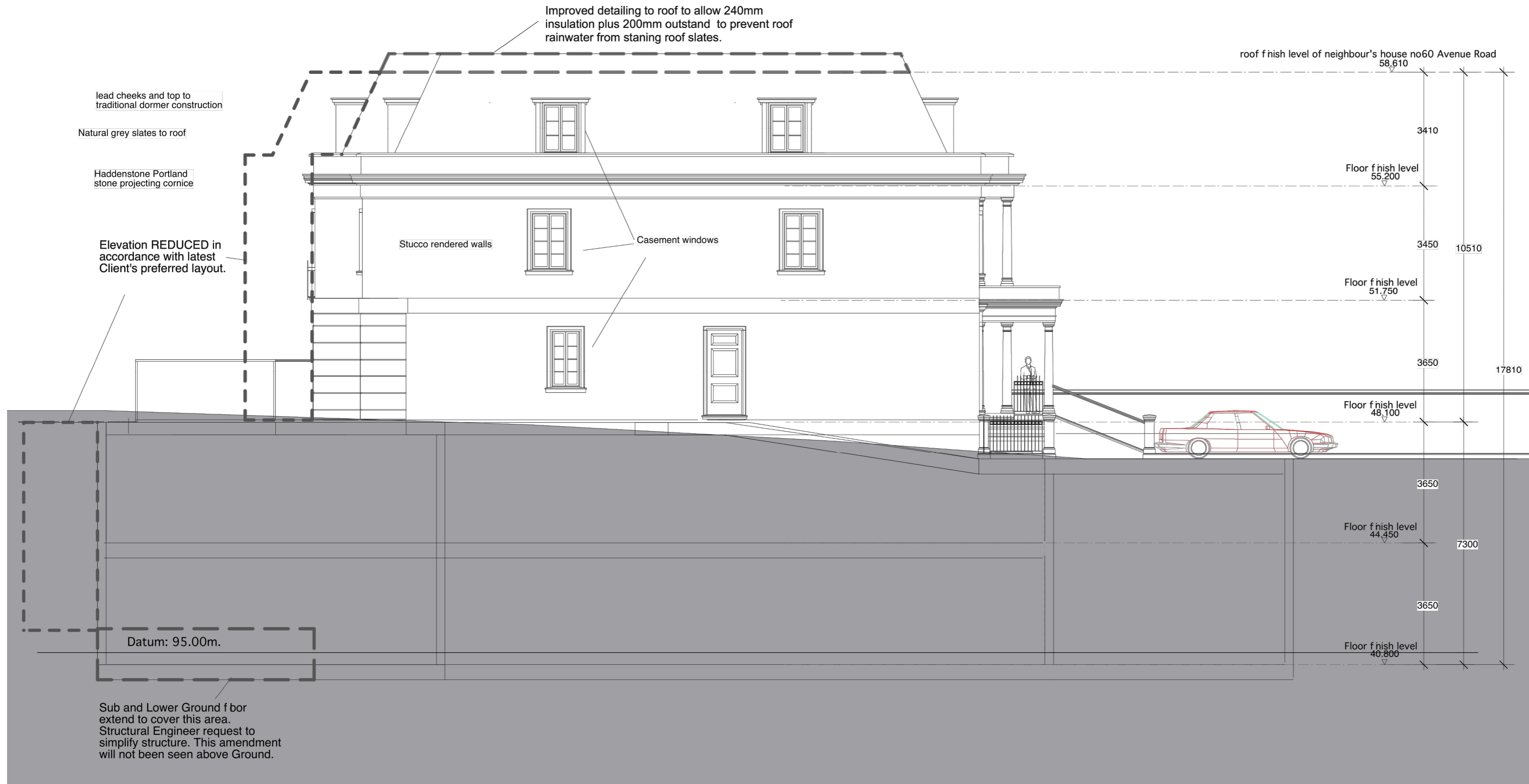
SIDE ELEVATION
