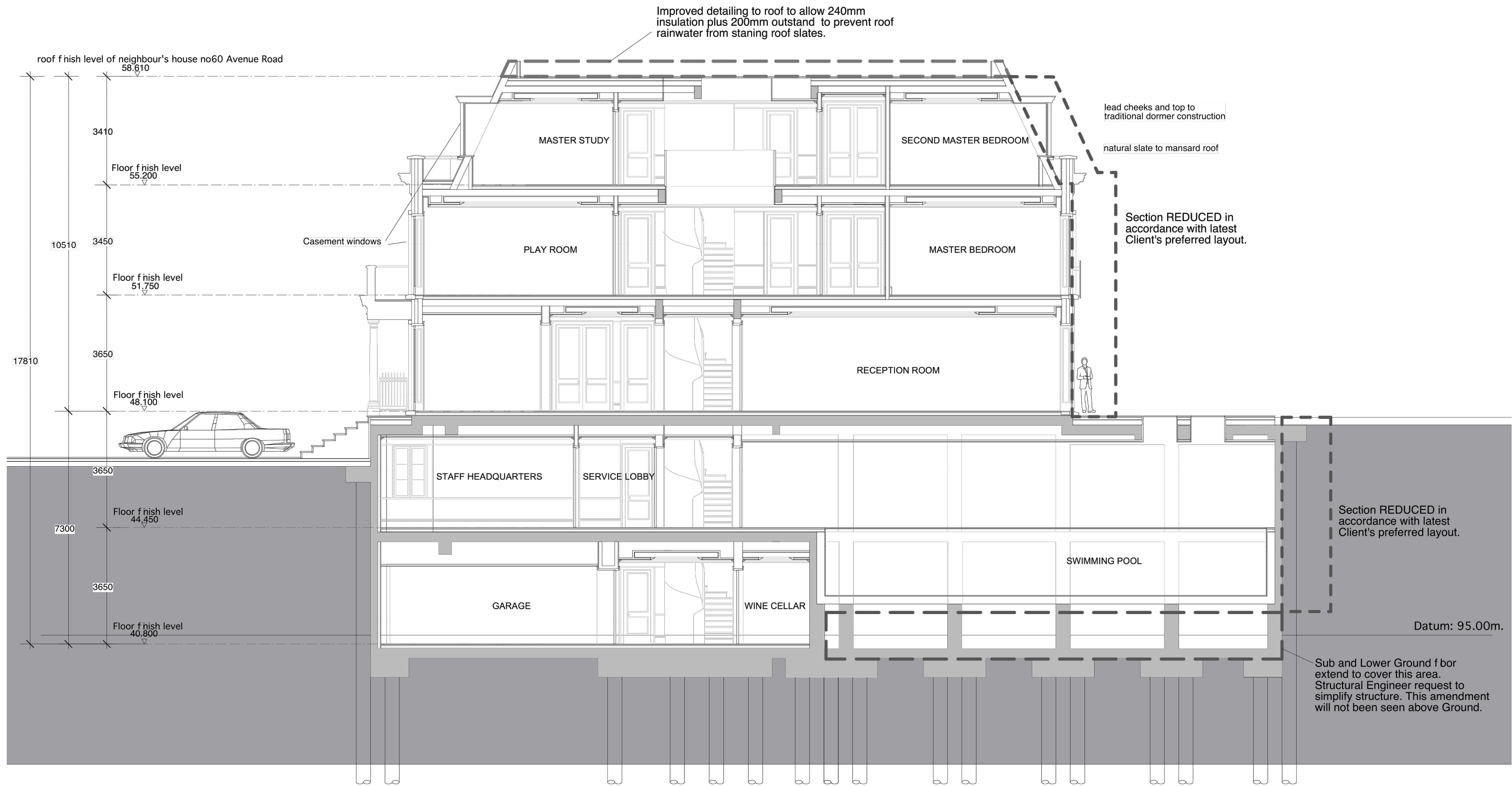
SECTION B - B
