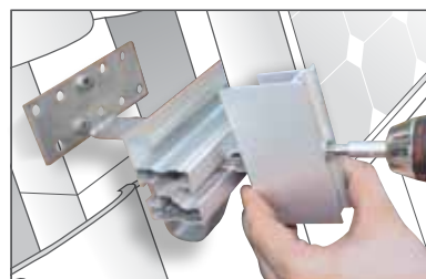
③ Snap in the Rapid 2+ clamp and screw it
