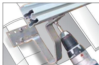
② Put on the rail and screw it
