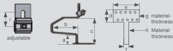
Dimensional drawing to the charts
