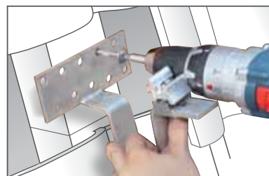
① Mount the roof hook
