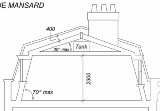
Figure 5. Mansard Roofs
