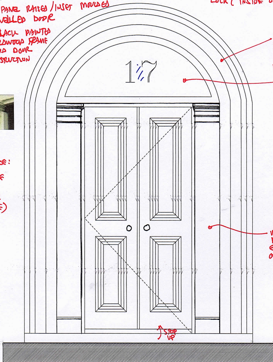
EXTERNAL ELEVATION
