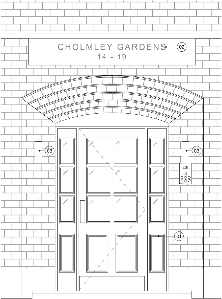
01 A160 ELEVATION DOOR 7_14-19 SCALE 1:25
