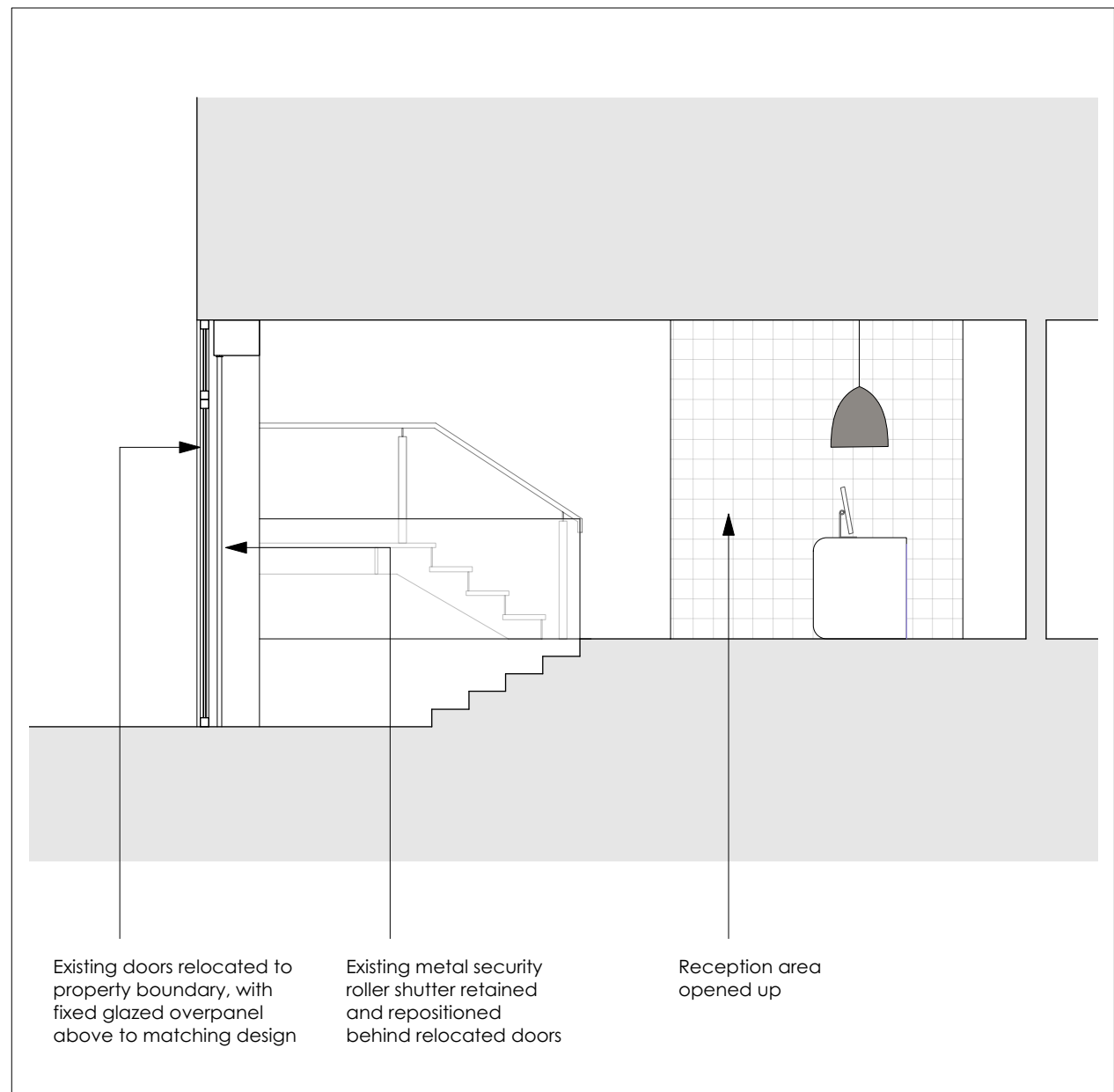
B Proposed Entrance Section GE.03 1:50
