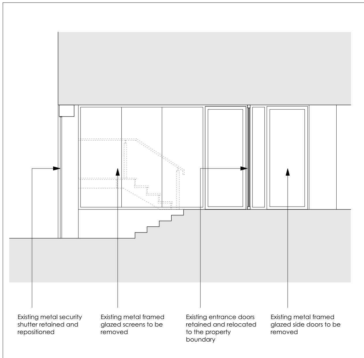
A Existing Entrance Section GE.03 1:50
