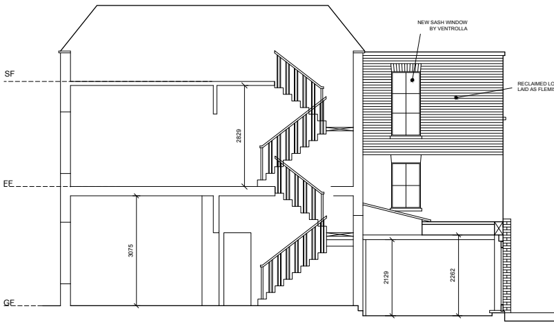
PROPOSED SIDE ELEVATION AND CROSS SECTION 1:50
