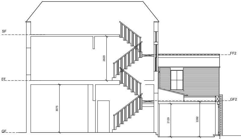
EXISTING SIDE ELEVATION AND CROSS SECTION 1:50
