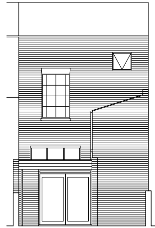
EXISTING REAR ELEVATION 1:50
