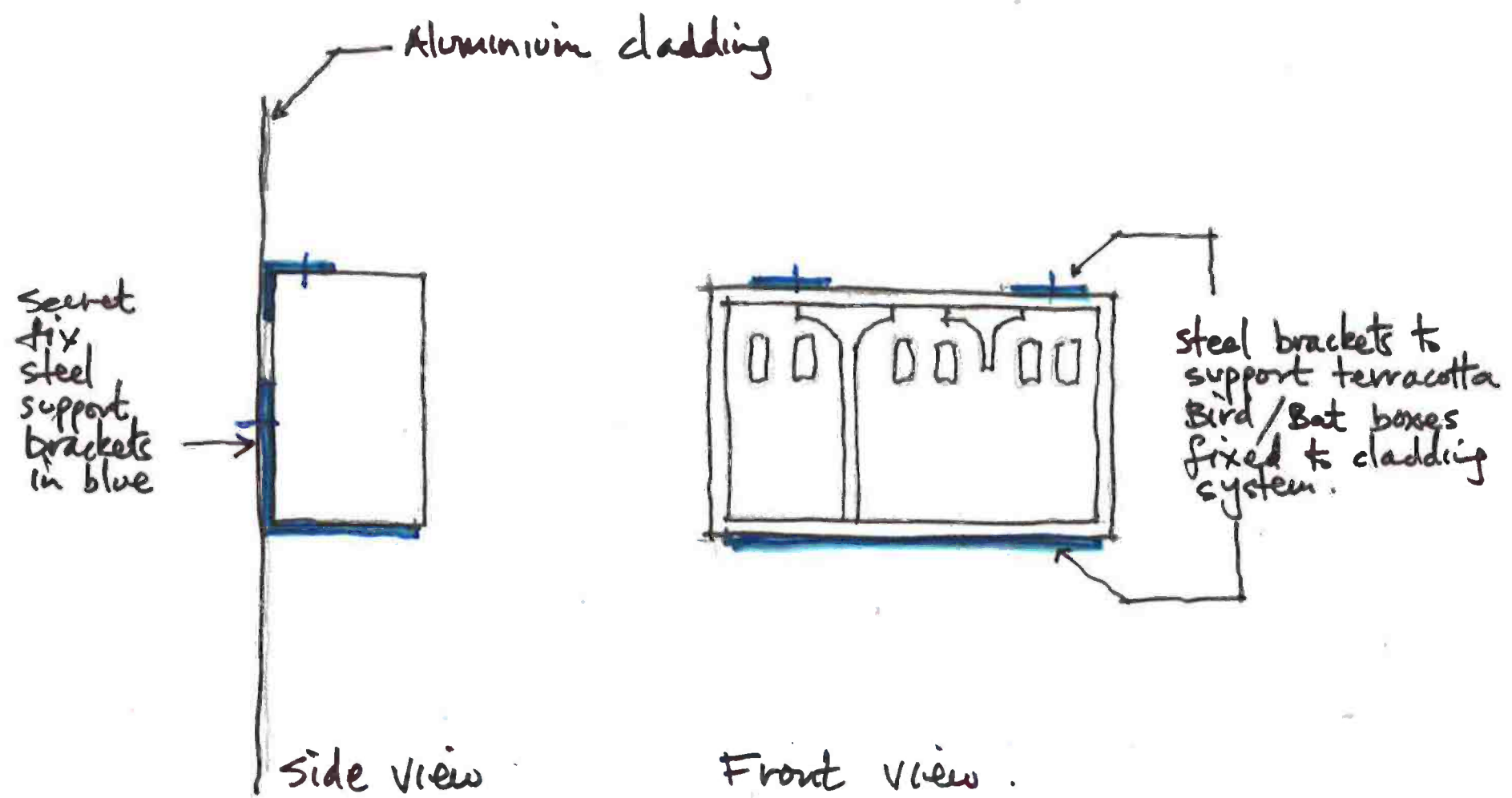
4 Pancras Square - Surface Bird/Bat boxes.
