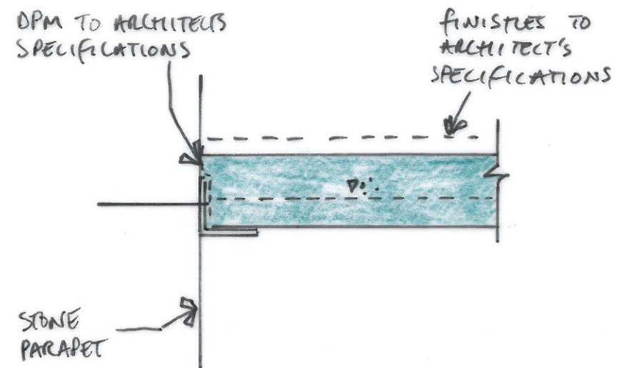
SECTION A-A (1:10)
