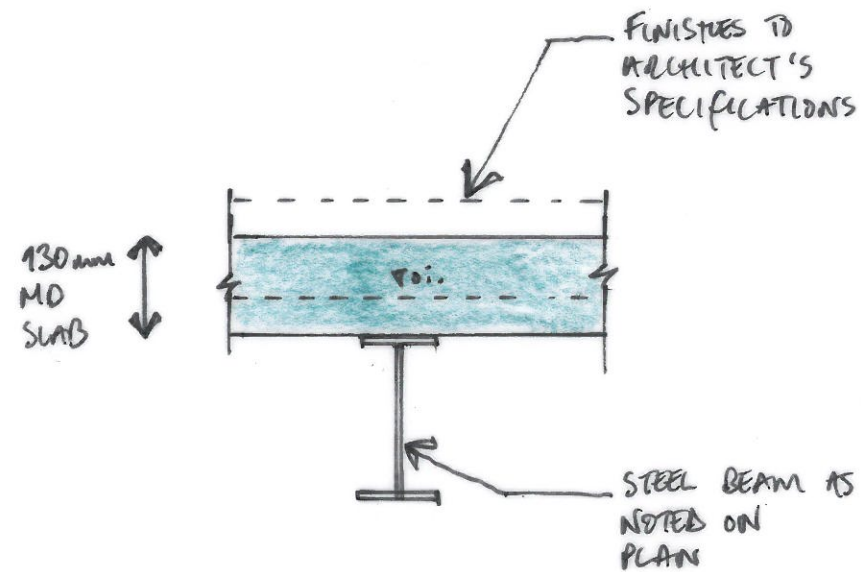
SECTION A-A (1:10)
