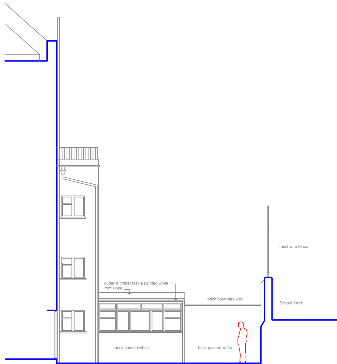
EXISTING PATIO ELEVATION
