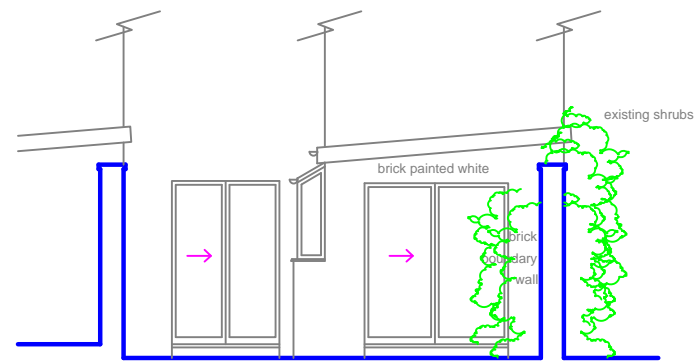
EXISTING SECTION
