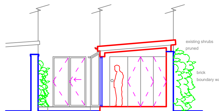
PROPOSED SECTION
