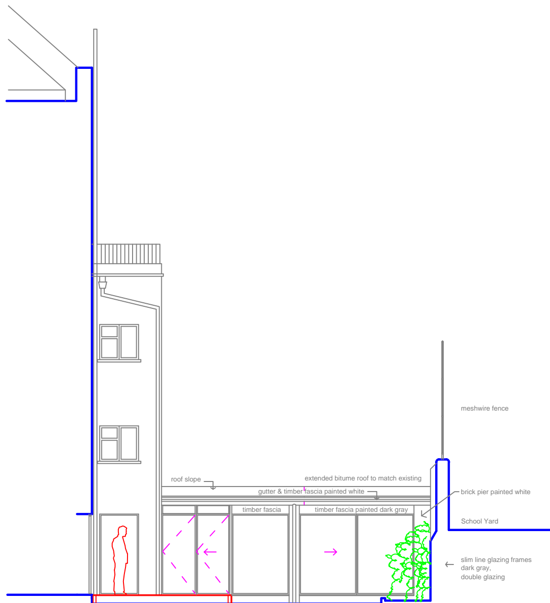
PROPOSED PATIO ELEVATION
