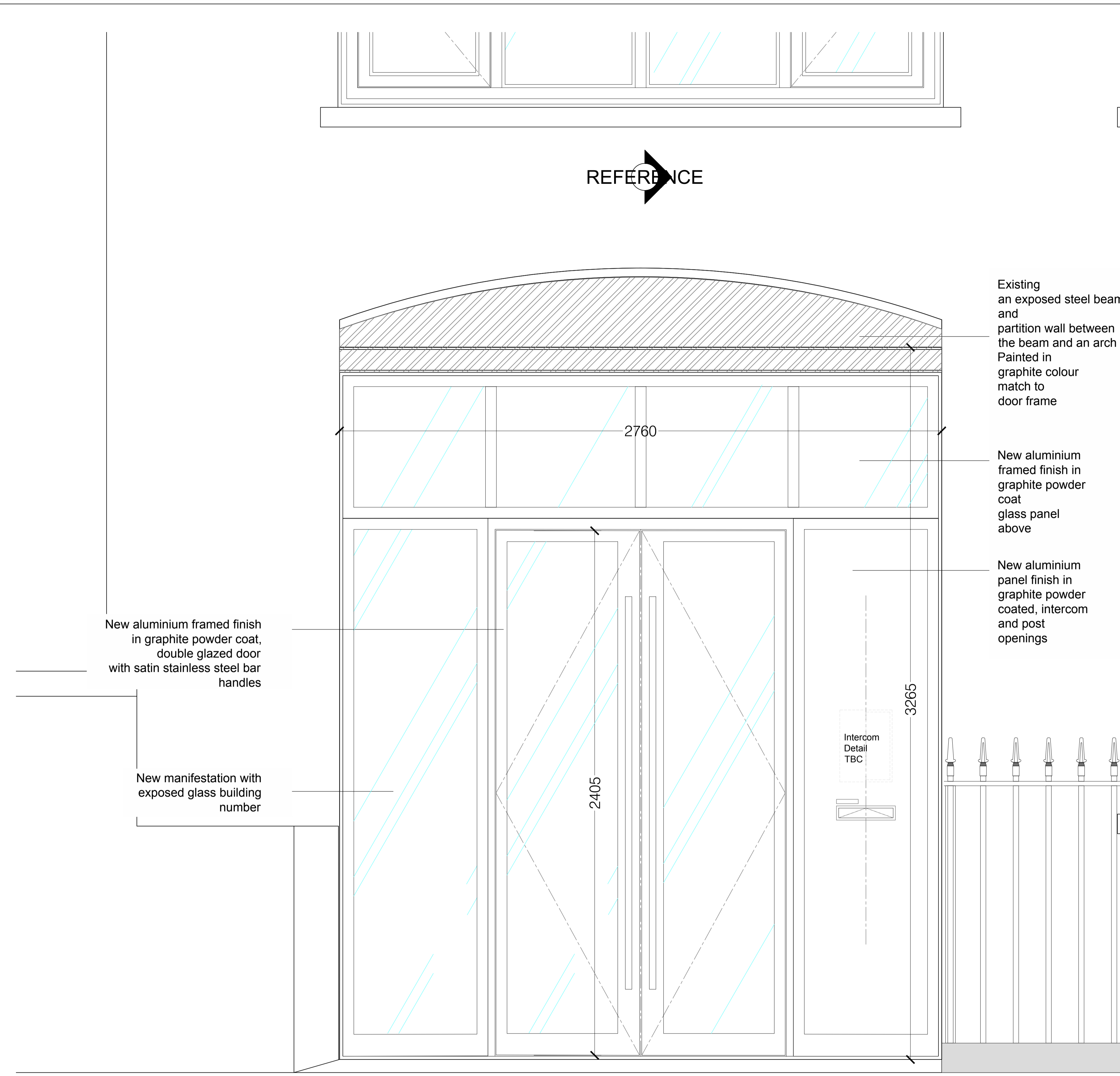
A ELEVATION Scale 1:25
