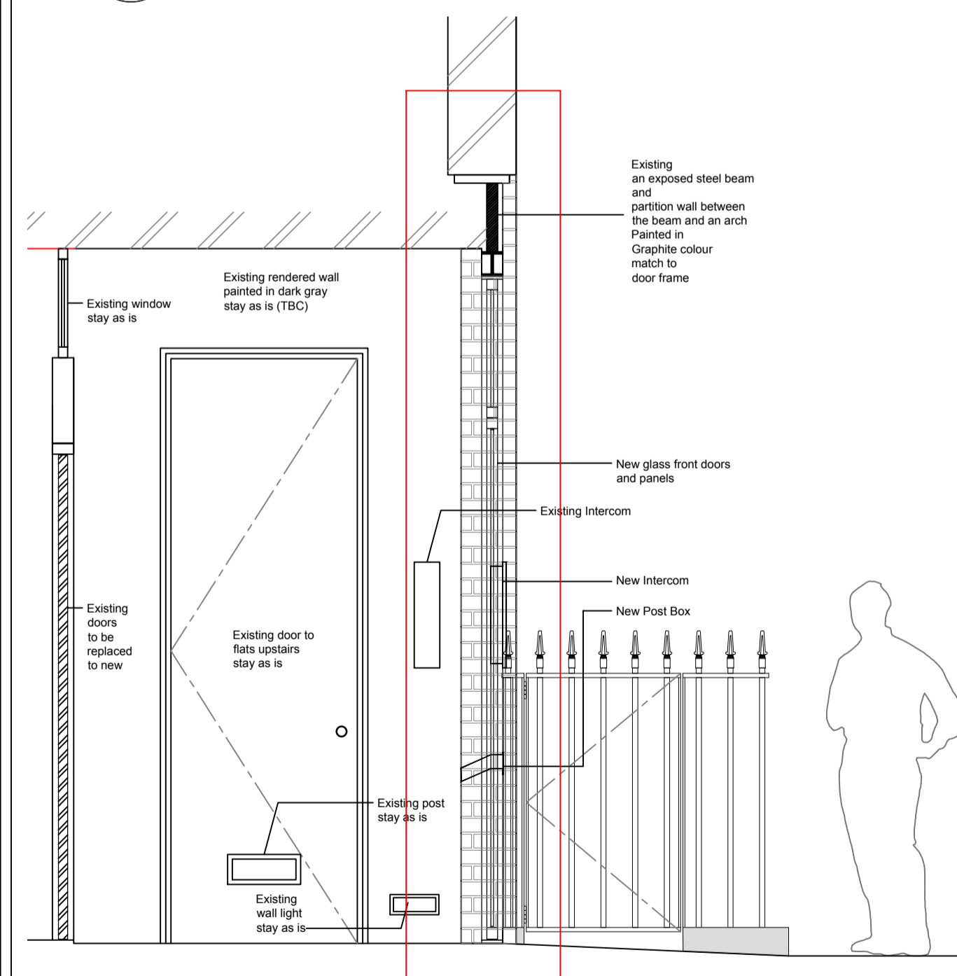
B SECTION Scale 1:25
