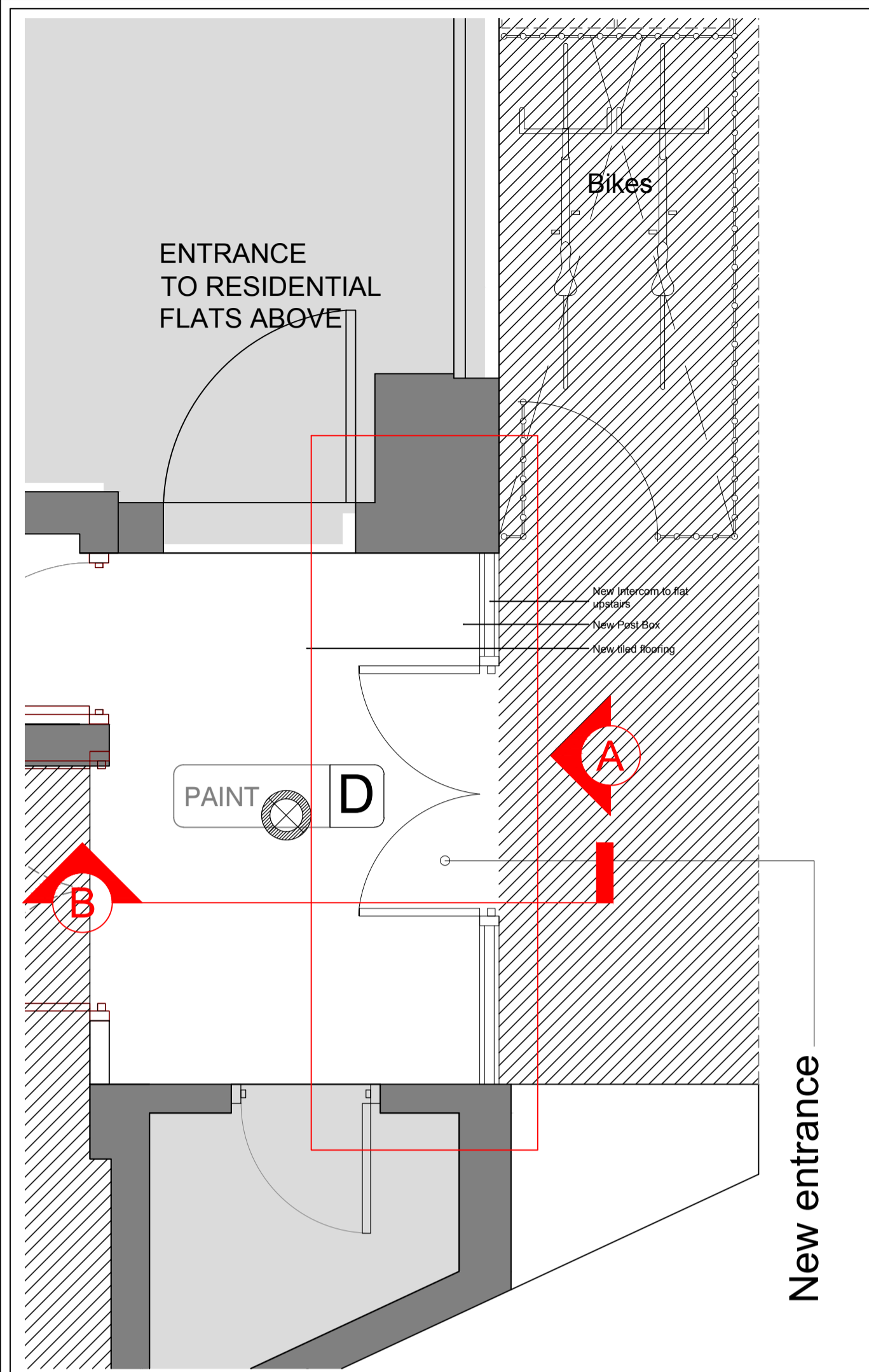
PLAN Scale 1:50
