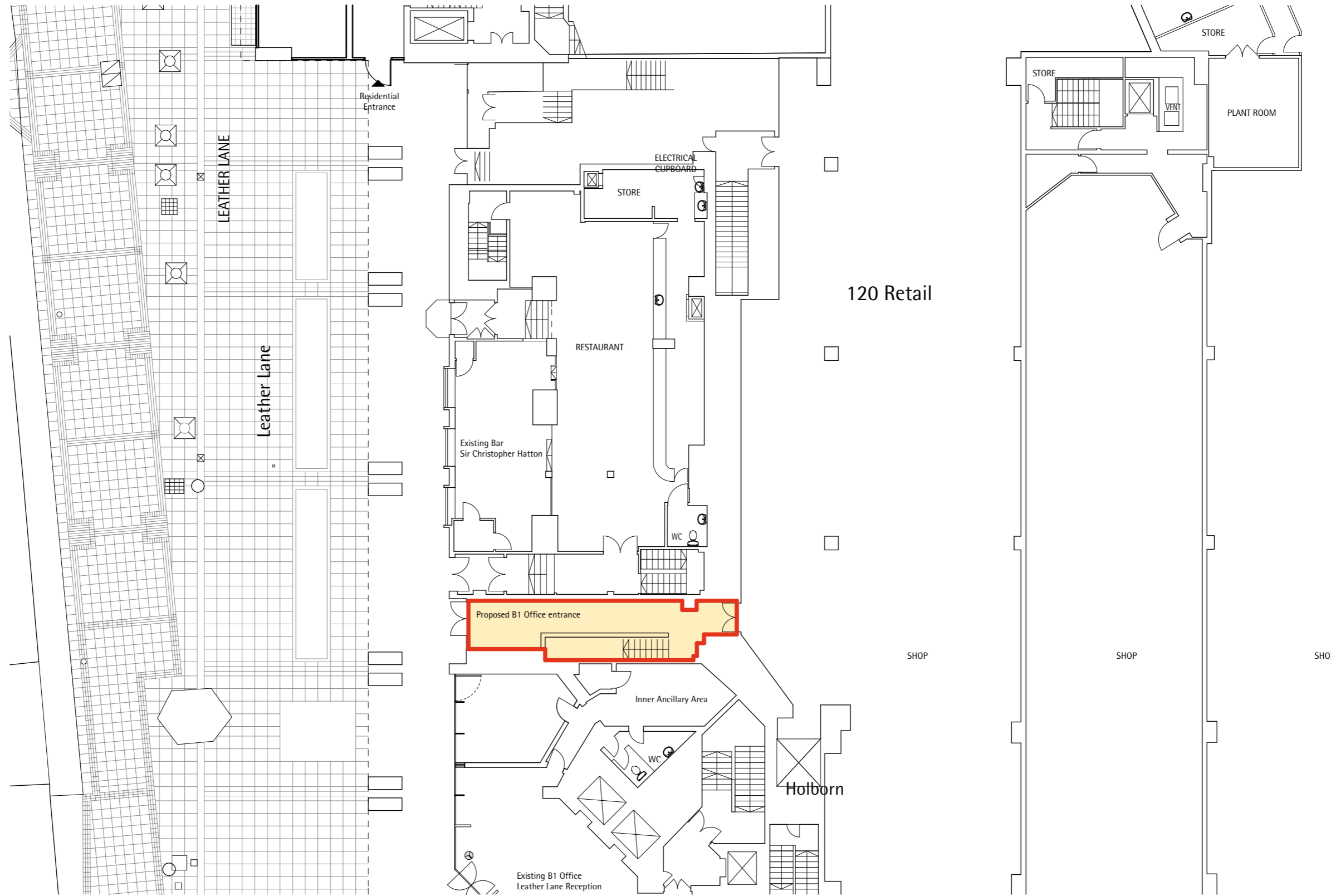
1 Proposed Ground Floor Plan SCALE 1:200
