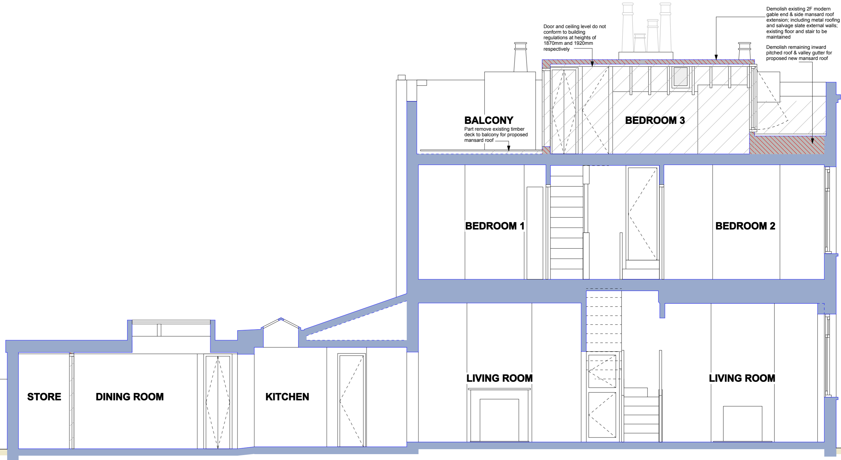
Section AA : Existing Scale 1:50
