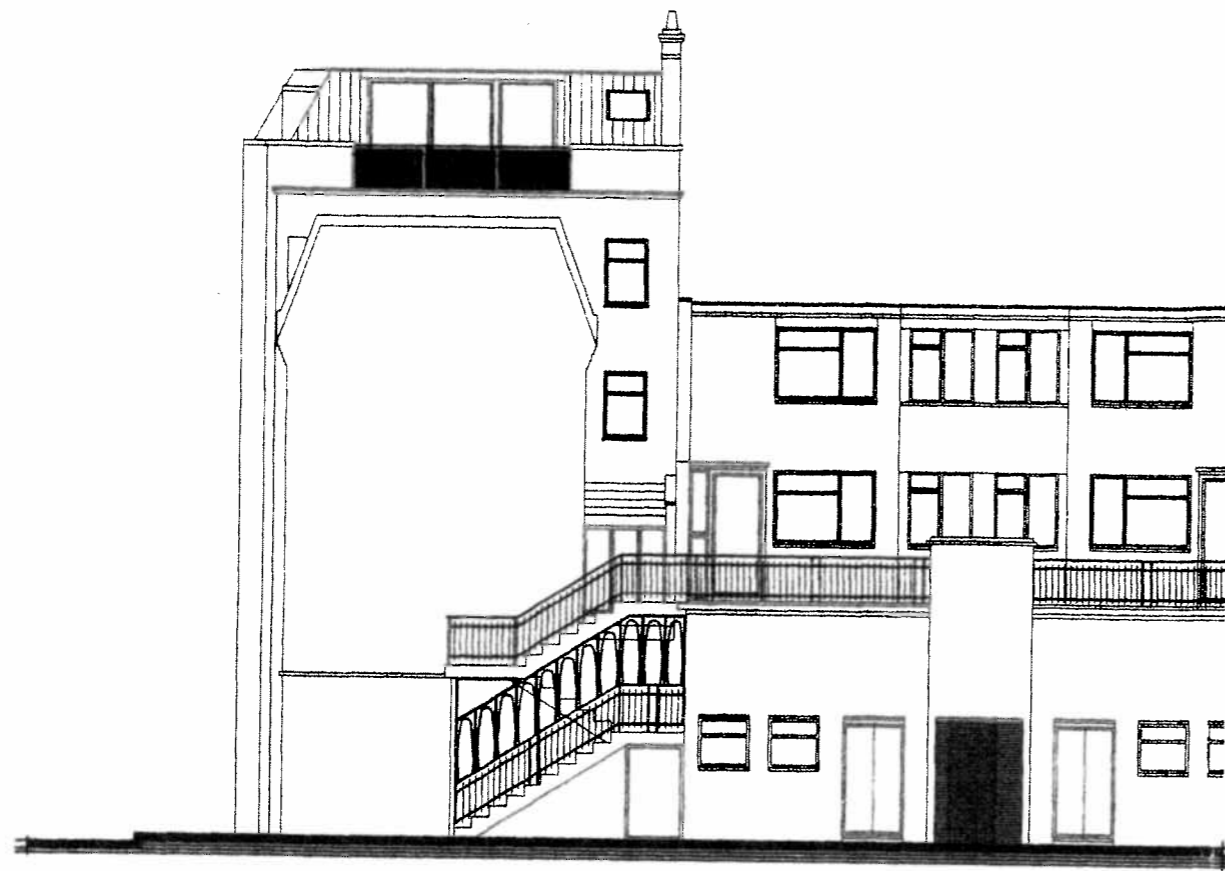
REAR ELEVATION 1:100
