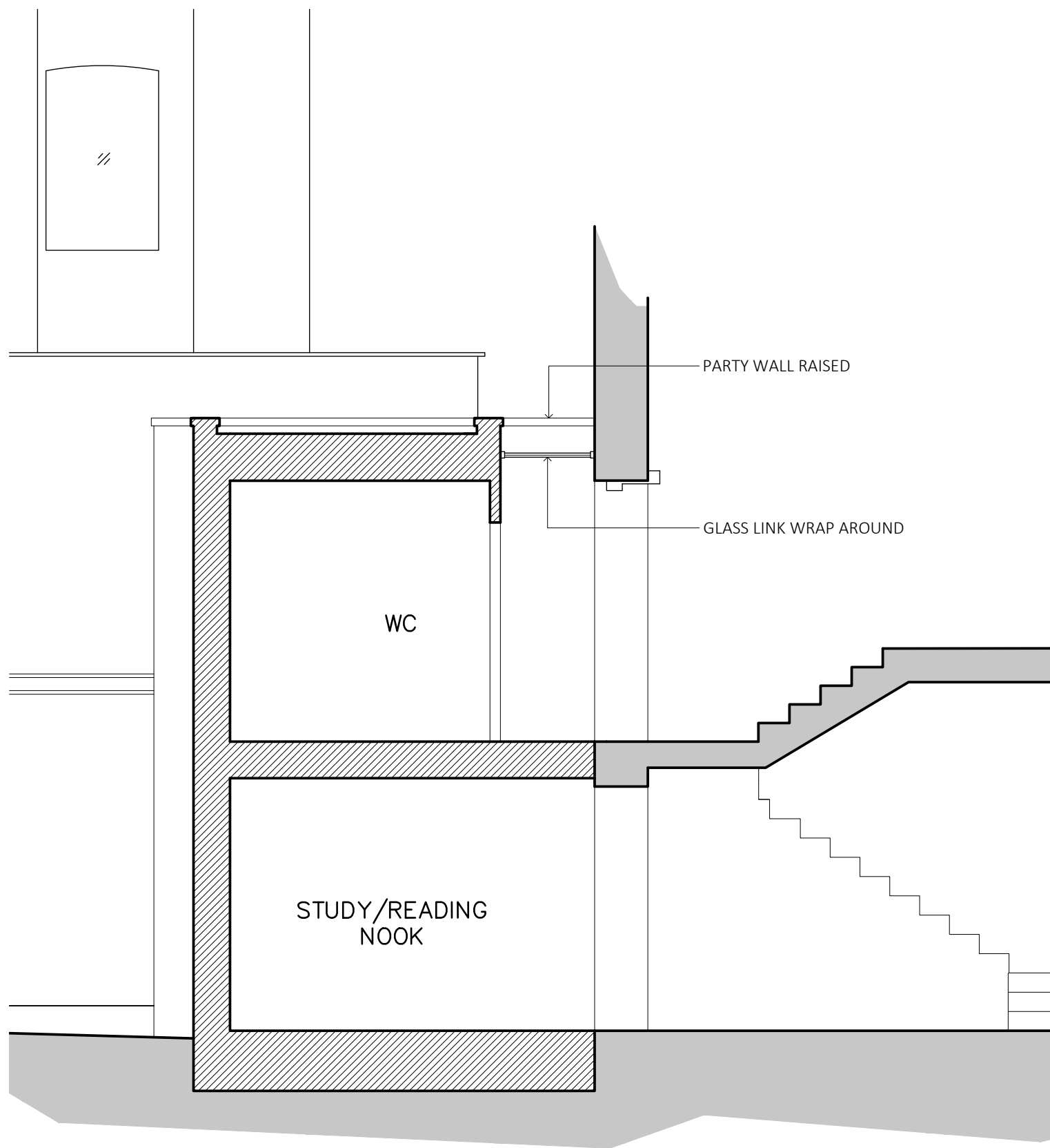
SECTION B-B
