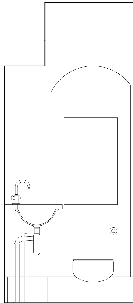
13RmB/10 - NORTH WALL
