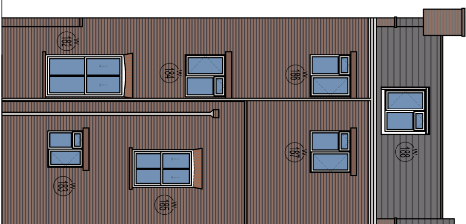
North Elevation
