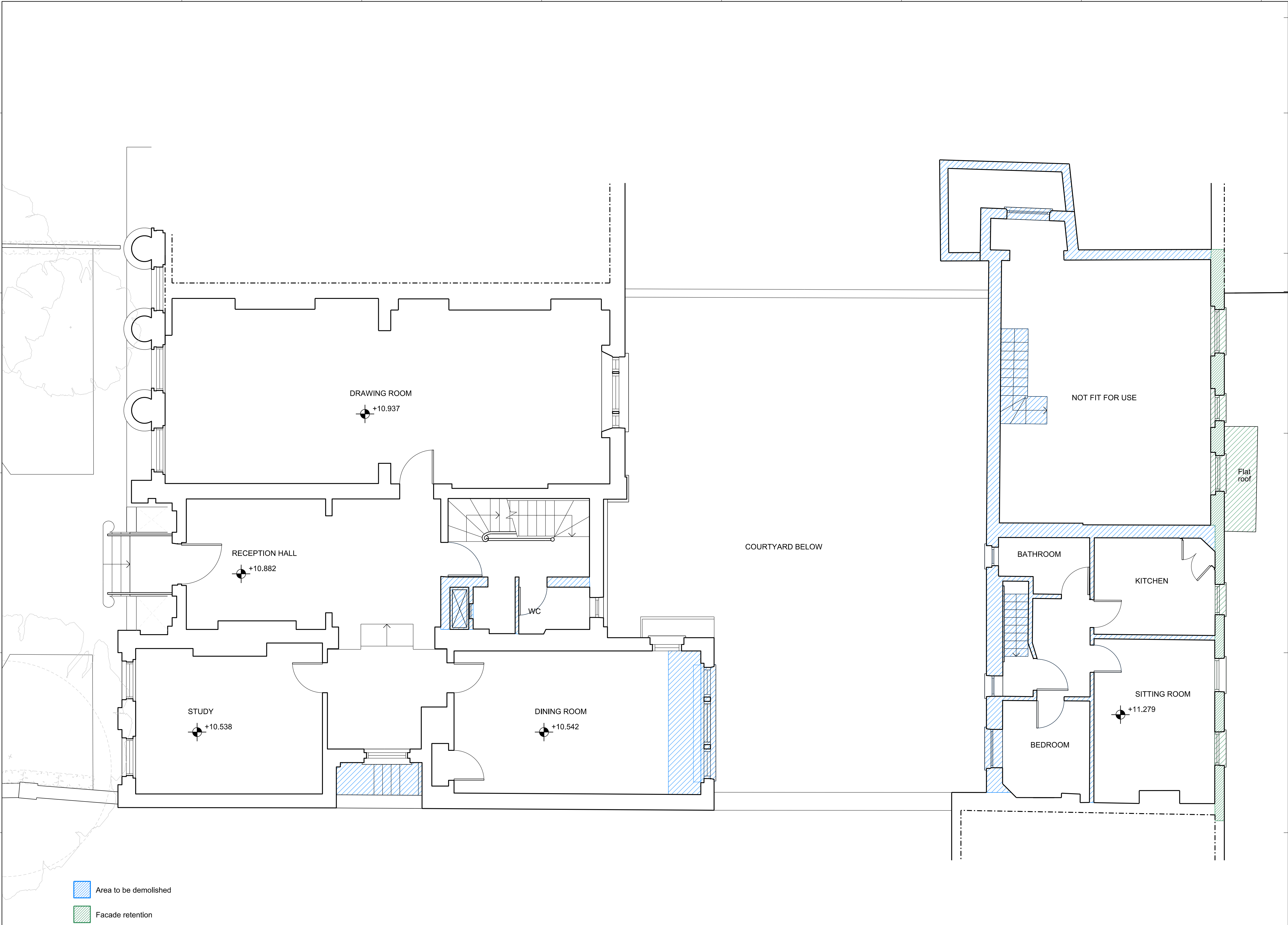
01 Demolition ground floor plan
